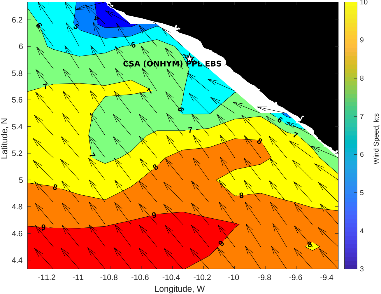
GFS Winds (kts) for CSA (ONHYM) PPL EBS - Liberia at 26-Nov-2025 09:00:00
