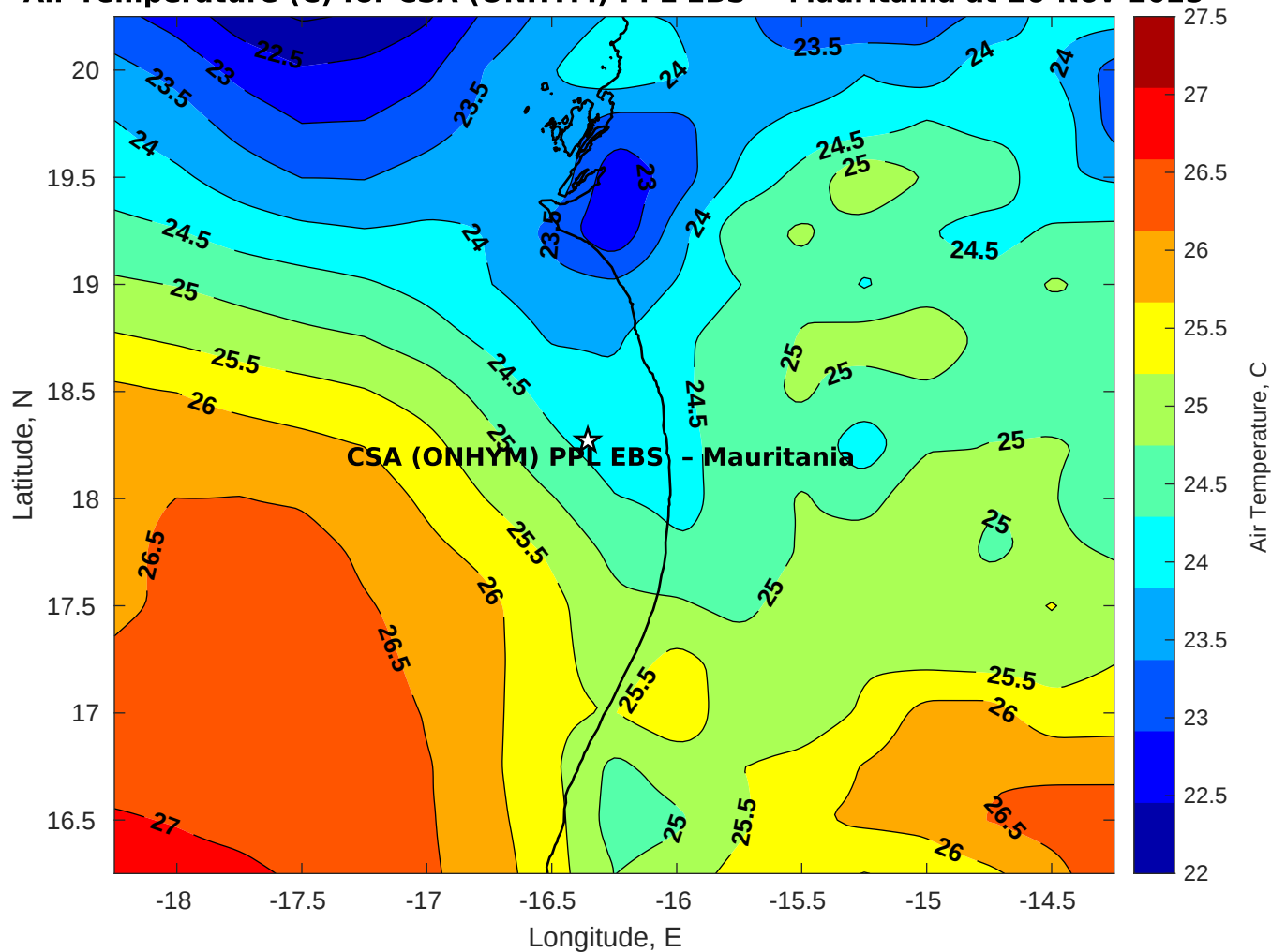
Air Temperature (C) for CSA (ONHYM) PPL EBS - Mauritania at 26-Nov-2025
