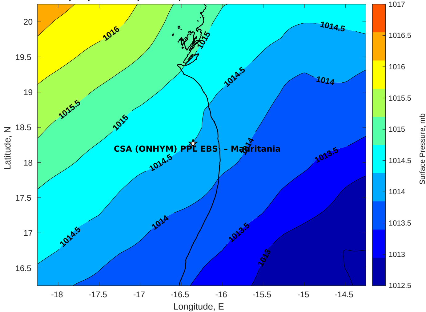
Surface Pressure (mb) for CSA (ONHYM) PPL EBS - Mauritania at 28-Nov-2025 00:00:00
