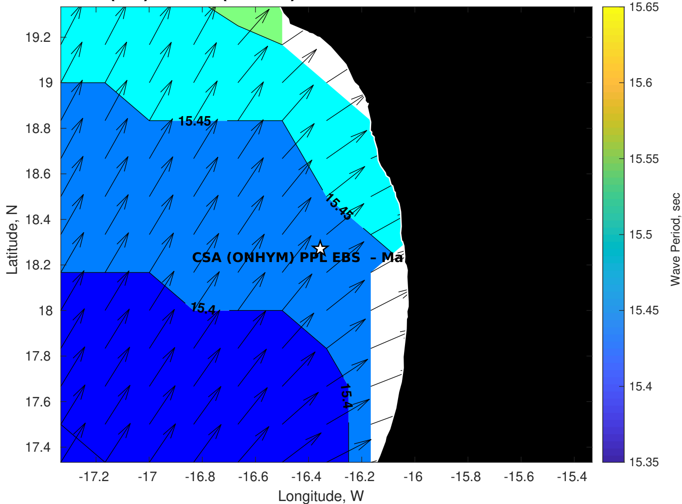
GFS Wave Period (sec) for CSA (ONHYM) PPL EBS - Mauritania at 26-Nov-2025 09:00:00
