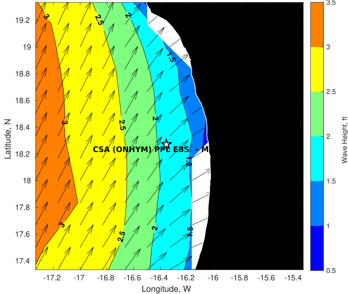
GFS Wave Height (ft) for CSA (ONHYM) PPL EBS - Mauritania at 26-Nov-2025 09:00:00
