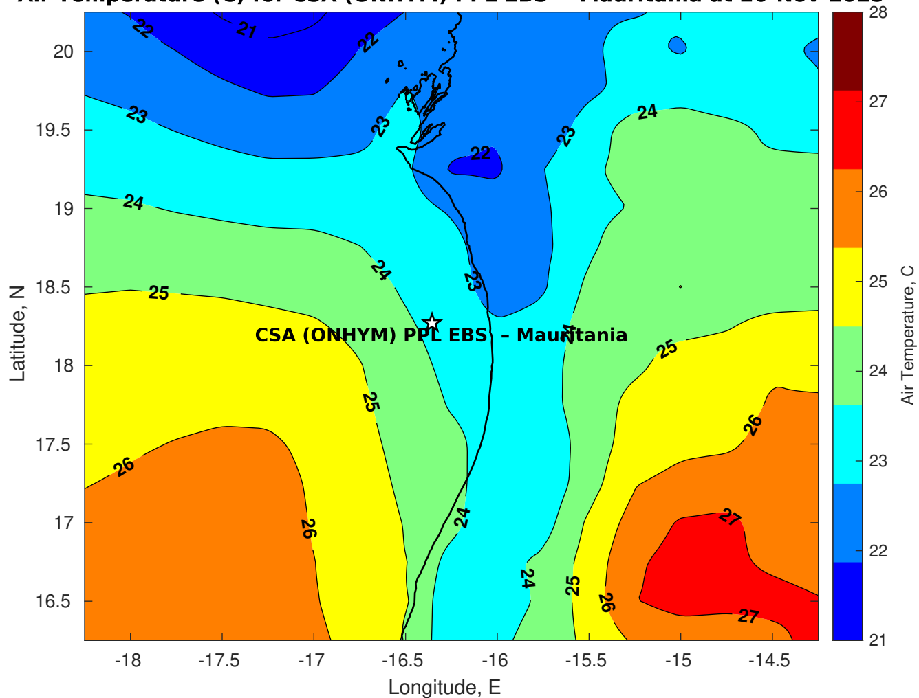
Air Temperature (C) for CSA (ONHYM) PPL EBS - Mauritania at 26-Nov-2025
