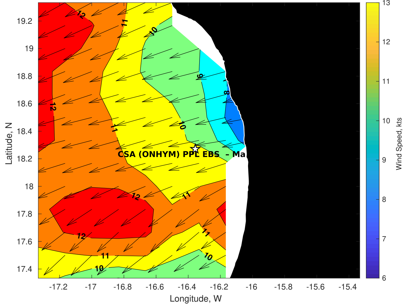
GFS Winds (kts) for CSA (ONHYM) PPL EBS - Mauritania at 26-Nov-2025 09:00:00
