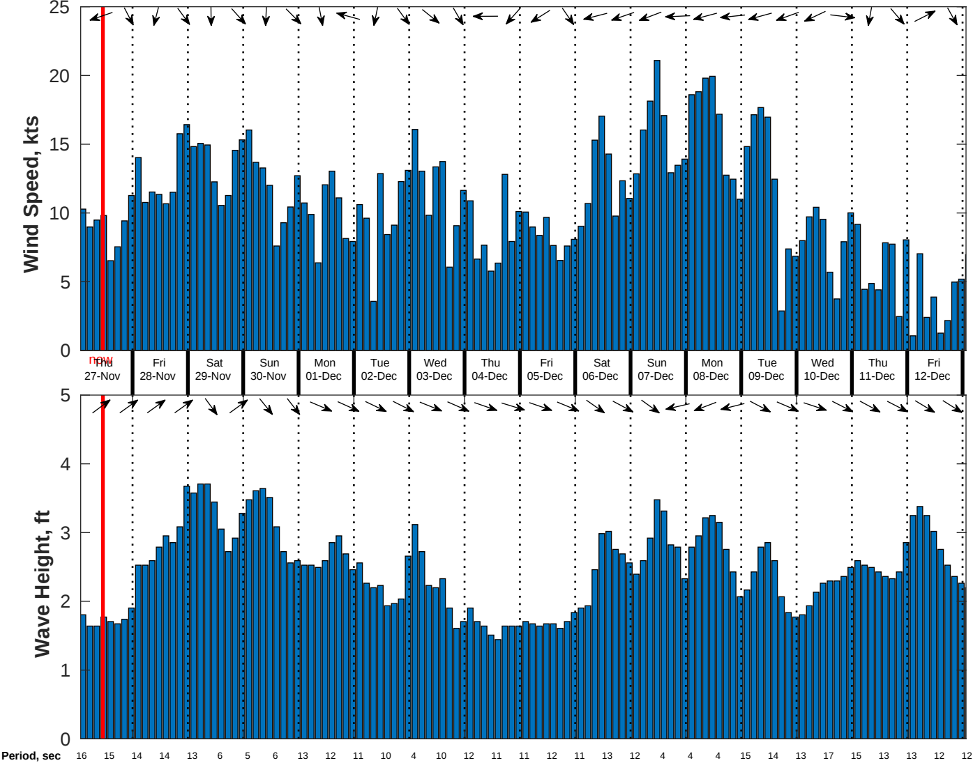
Wind & Wave Forecast for CSA (ONHYM) PPL EBS - Mauritania from 26-Nov-2025 01:00:00 to 12-Dec-2025 01:00:00
