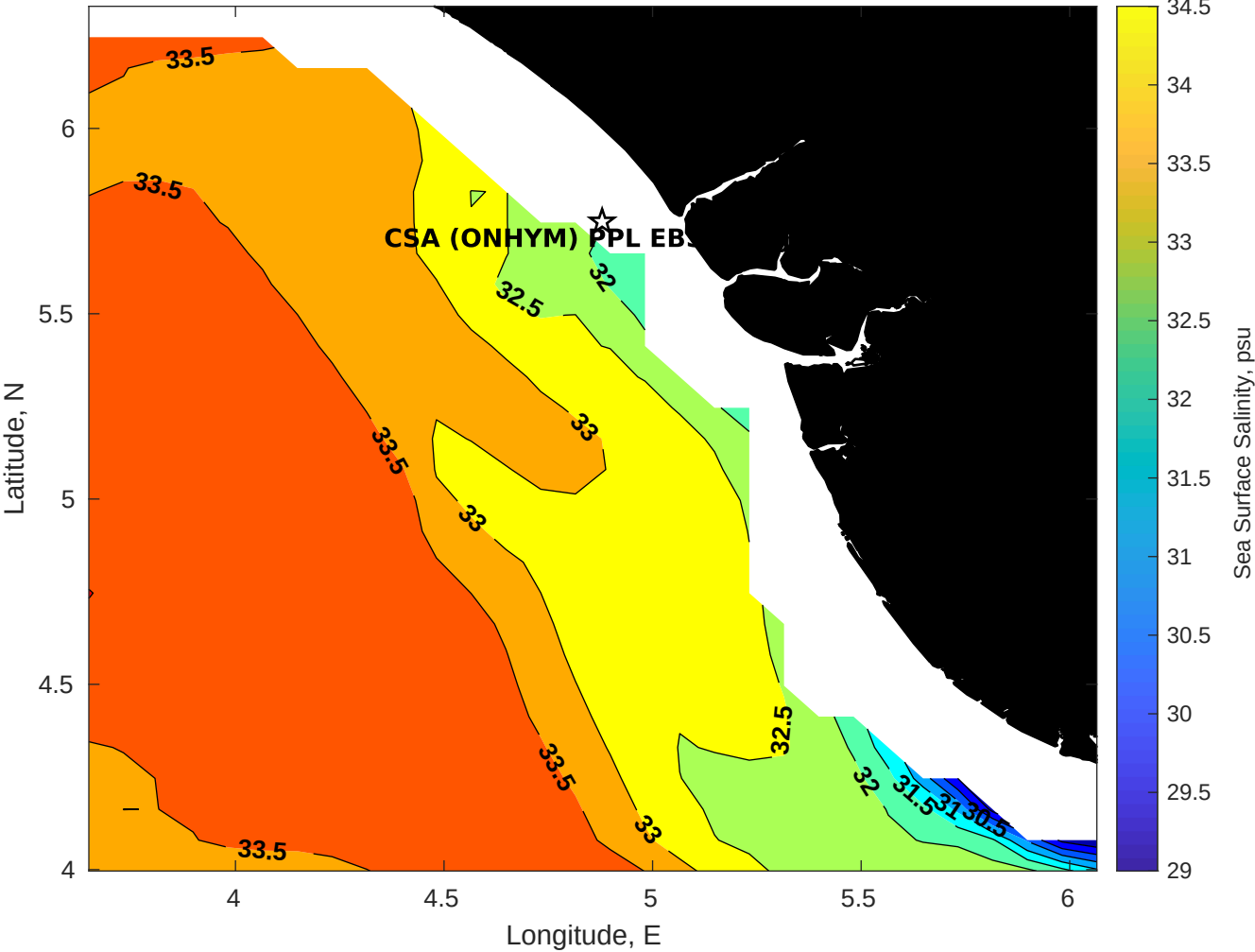
Surface Salinity for CSA (ONHYM) PPL EBS - Nigeria at 25-Nov-2025 00:00:00
