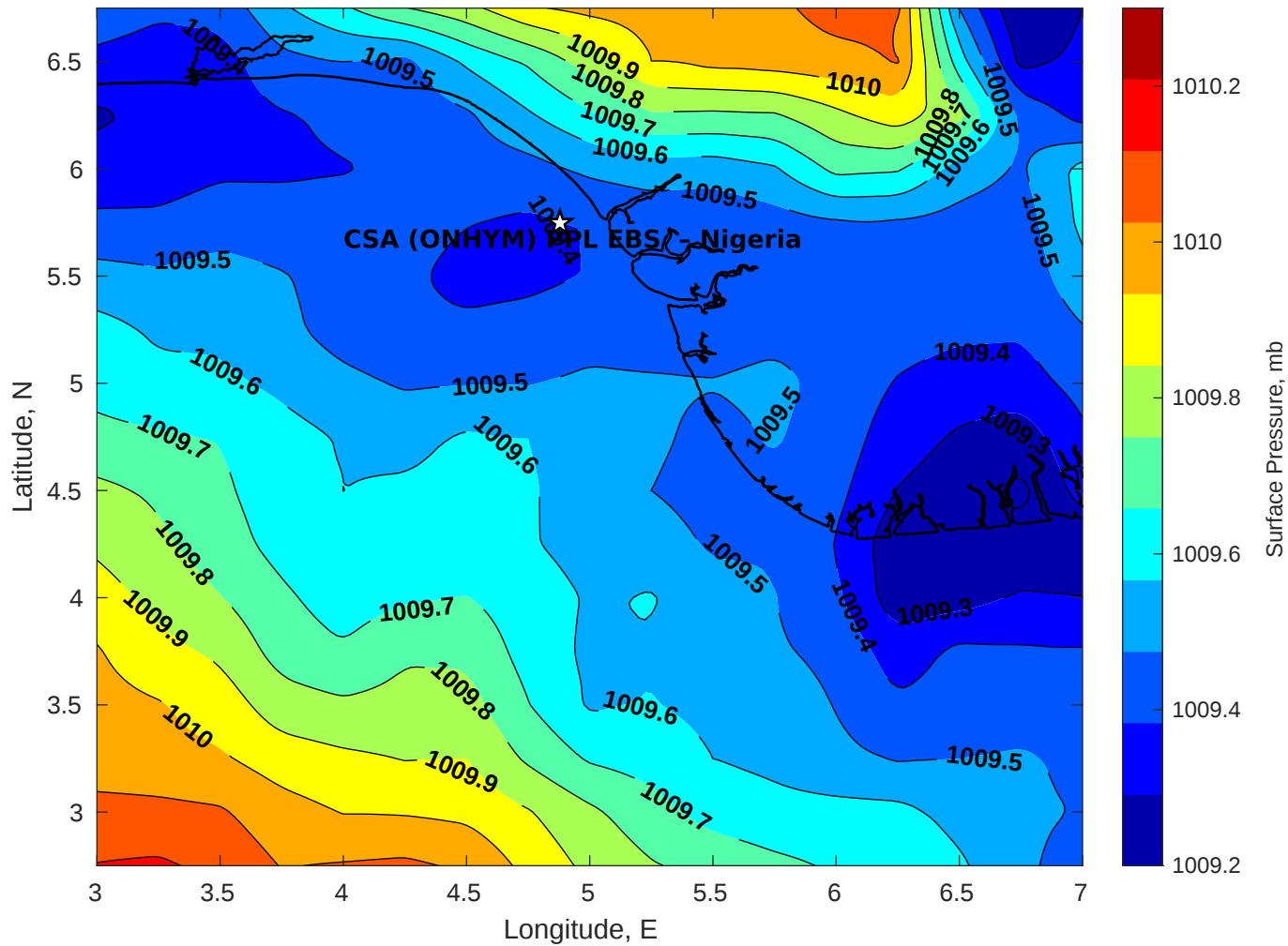
Surface Pressure (mb) for CSA (ONHYM) PPL EBS - Nigeria at 26-Nov-2025 00:00:00
