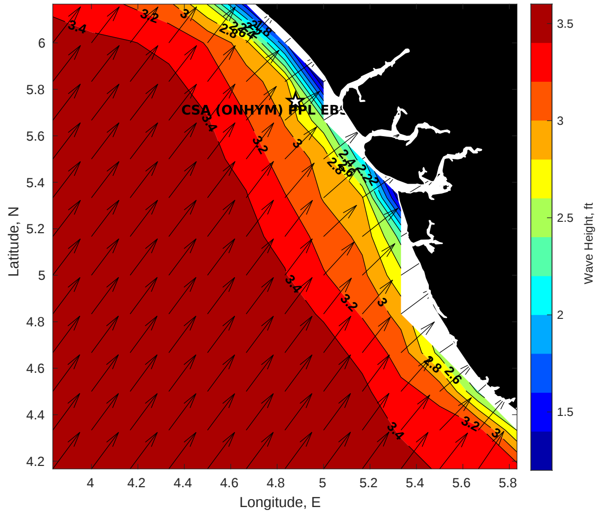
GFS Wave Height (ft) for CSA (ONHYM) PPL EBS - Nigeria at 26-Nov-2025 09:00:00
