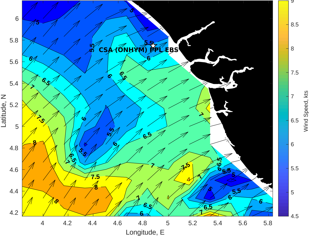
GFS Winds (kts) for CSA (ONHYM) PPL EBS - Nigeria at 26-Nov-2025 09:00:00
