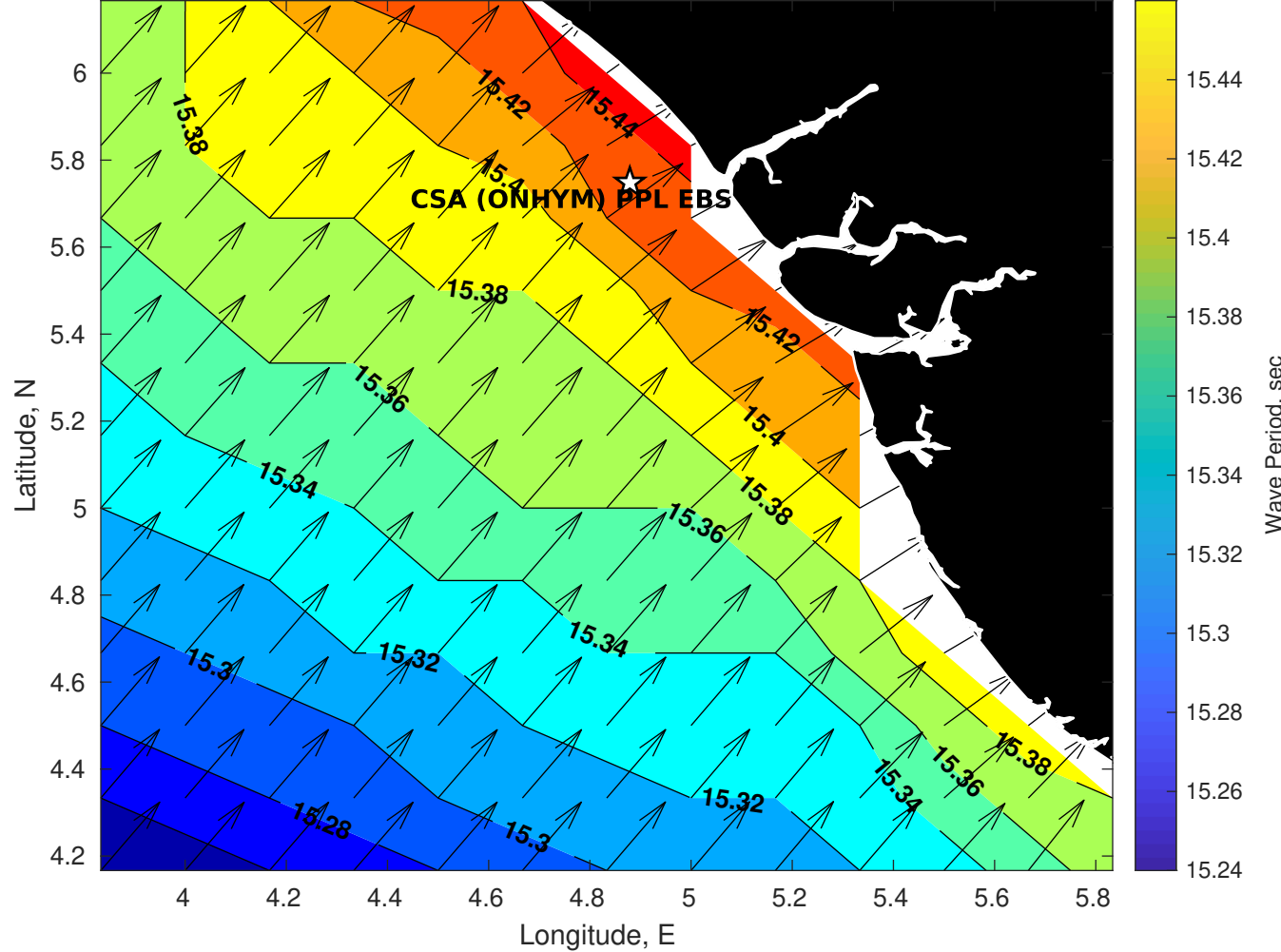
GFS Wave Period (sec) for CSA (ONHYM) PPL EBS - Nigeria at 26-Nov-2025 09:00:00
