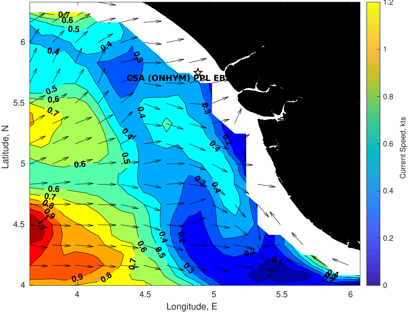
Surface Currents for CSA (ONHYM) PPL EBS - Nigeria at 25-Nov-2025 00:00:00
