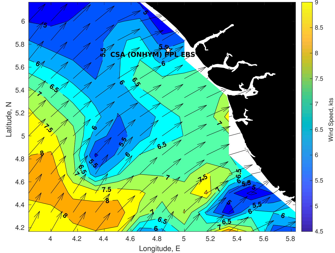
GFS Winds (kts) for CSA (ONHYM) PPL EBS - Nigeria at 26-Nov-2025 09:00:00
