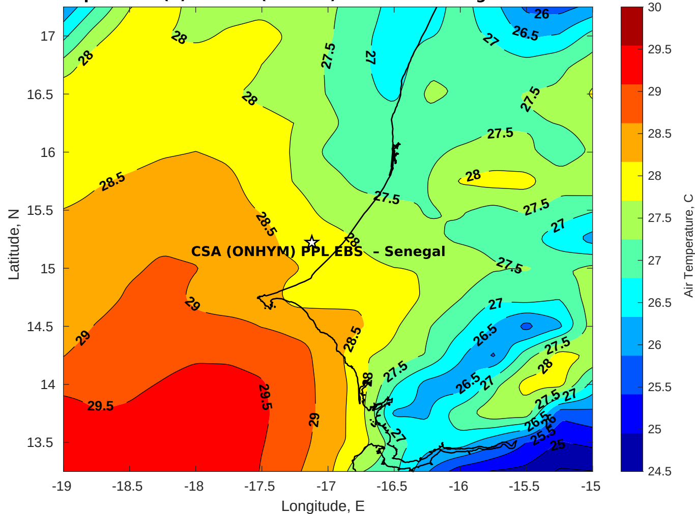
Air Temperature (C) for CSA (ONHYM) PPL EBS - Senegal at 26-Nov-2025
