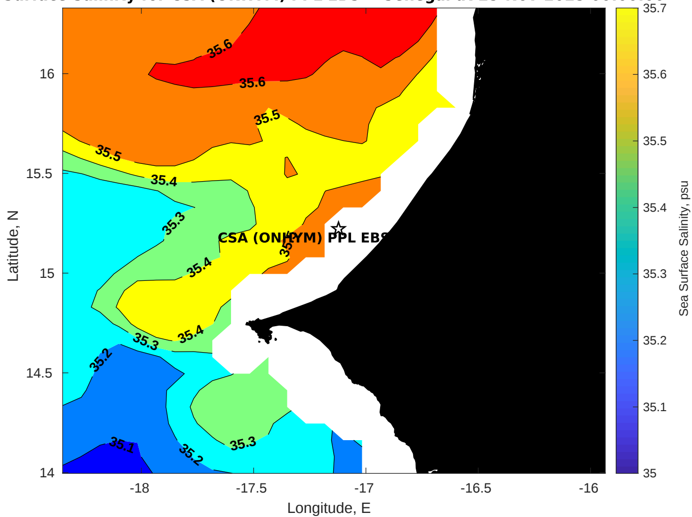
Surface Salinity for CSA (ONHYM) PPL EBS - Senegal at 25-Nov-2025 00:00:00
