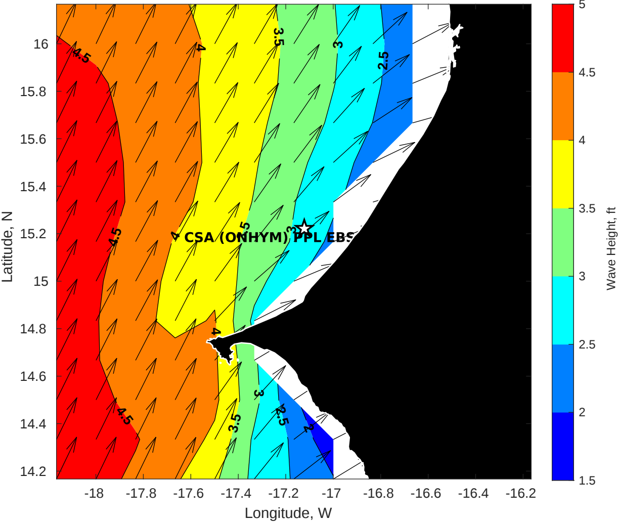
GFS Wave Height (ft) for CSA (ONHYM) PPL EBS - Senegal at 26-Nov-2025 09:00:00
