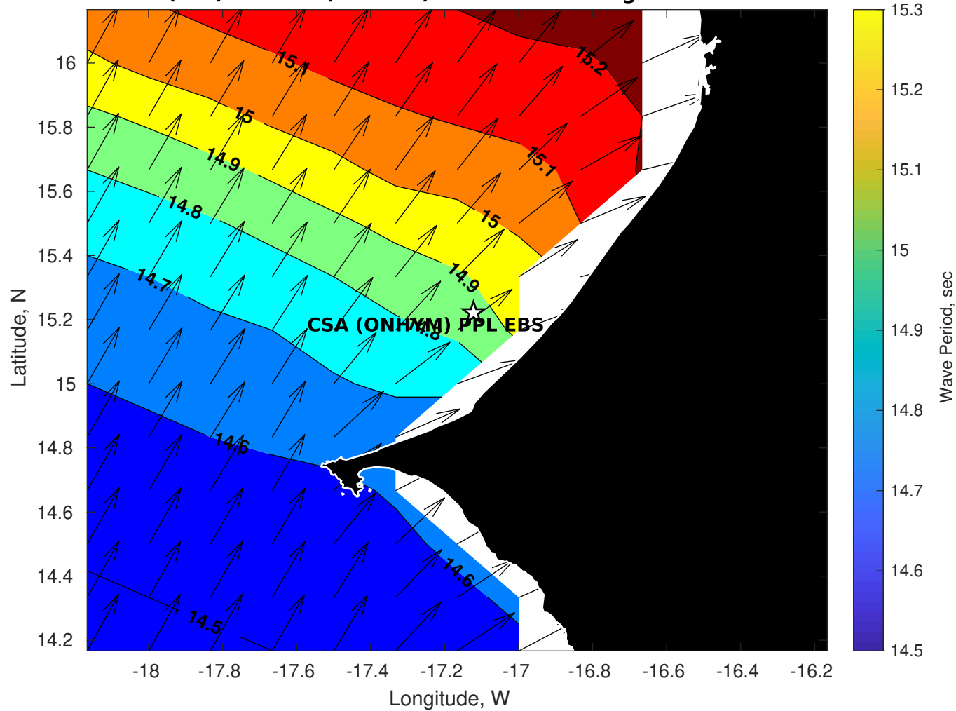
GFS Wave Period (sec) for CSA (ONHYM) PPL EBS - Senegal at 26-Nov-2025 09:00:00
