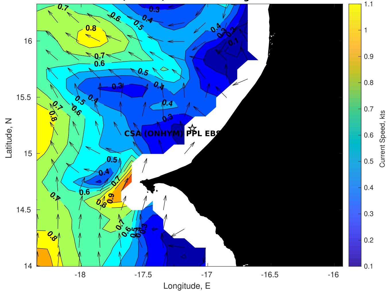
Surface Currents for CSA (ONHYM) PPL EBS - Senegal at 25-Nov-2025 00:00:00
