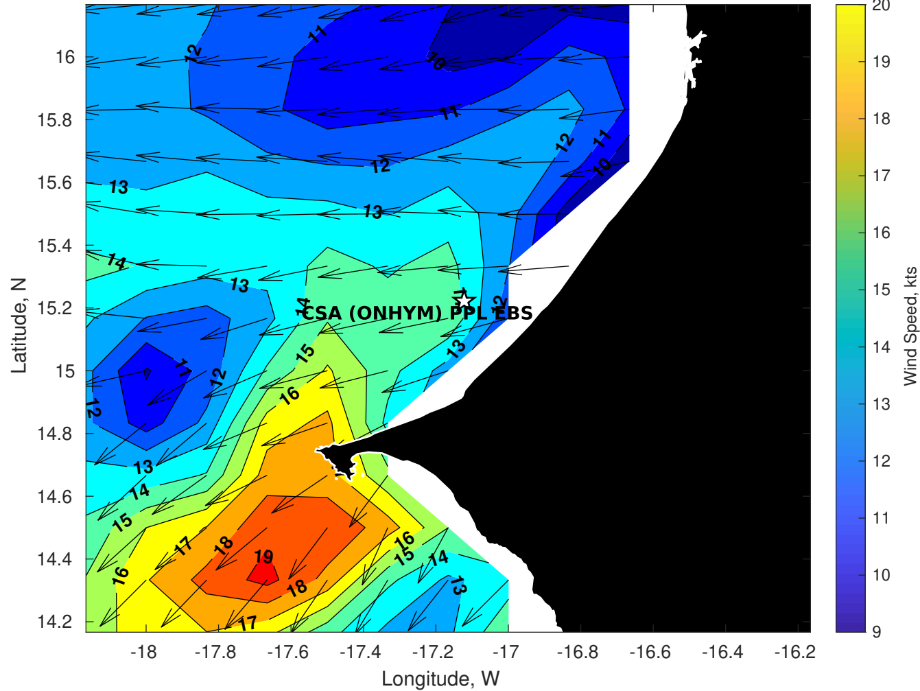
GFS Winds (kts) for CSA (ONHYM) PPL EBS - Senegal at 26-Nov-2025 09:00:00
