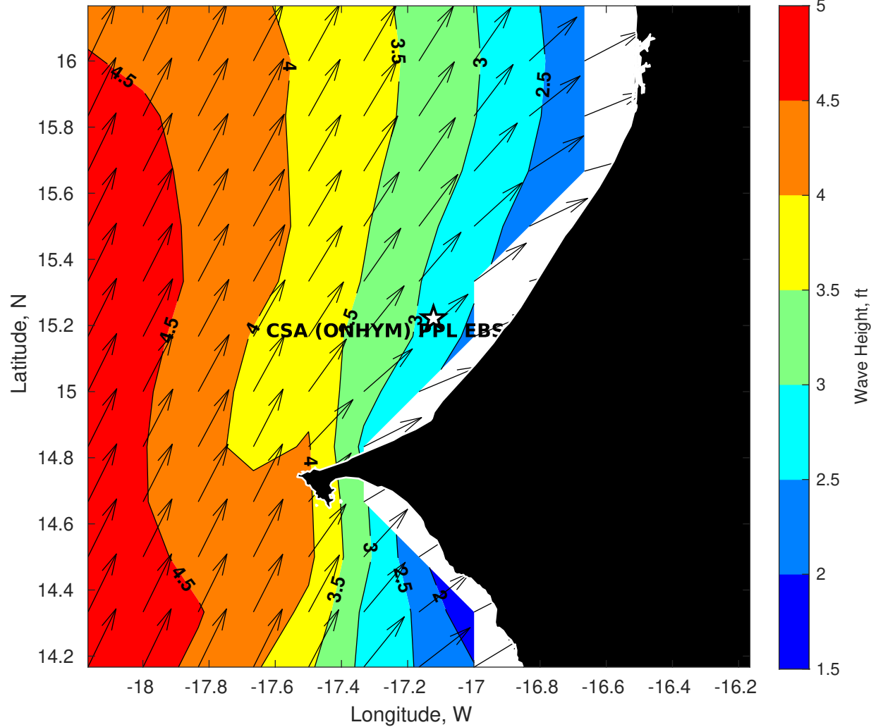
GFS Wave Height (ft) for CSA (ONHYM) PPL EBS - Senegal at 26-Nov-2025 09:00:00
