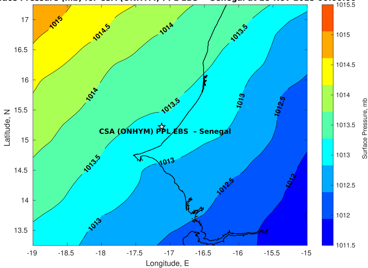
Surface Pressure (mb) for CSA (ONHYM) PPL EBS - Senegal at 28-Nov-2025 00:00:00
