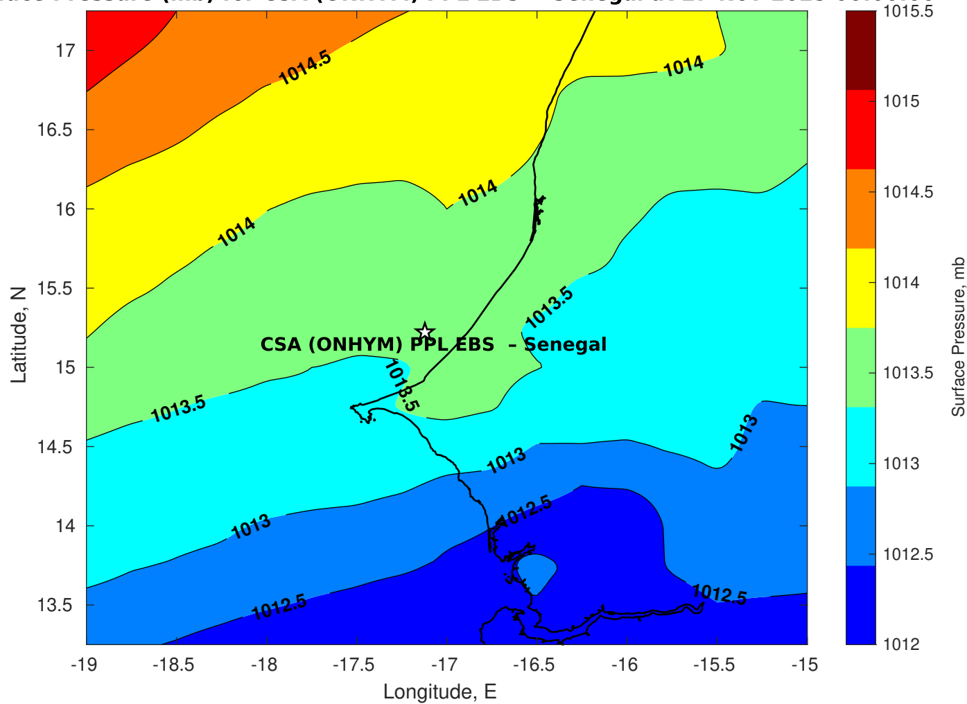
Surface Pressure (mb) for CSA (ONHYM) PPL EBS - Senegal at 27-Nov-2025 00:00:00
