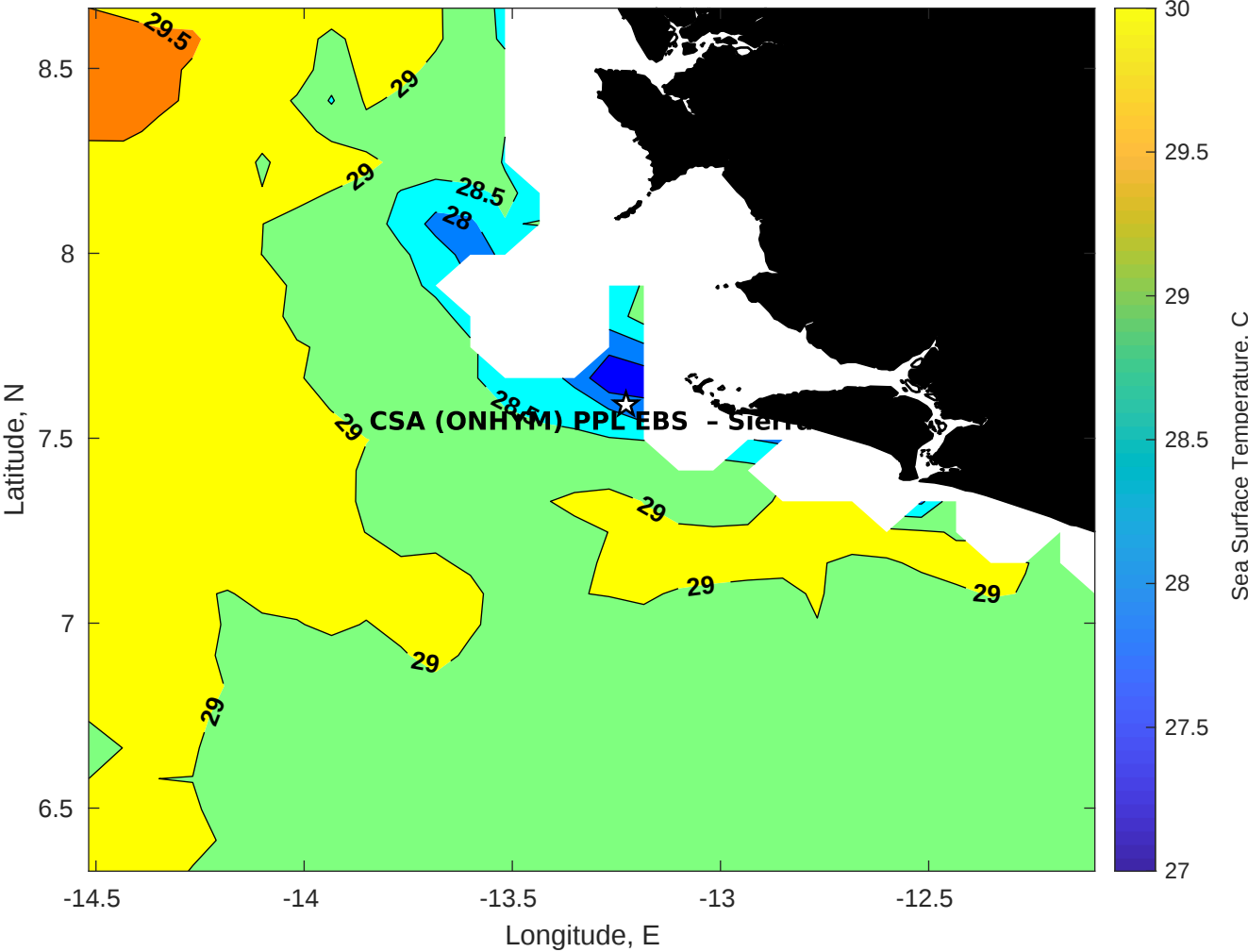
SST for CSA (ONHYM) PPL EBS - Sierra Leone at 25-Nov-2025 00:00:00
