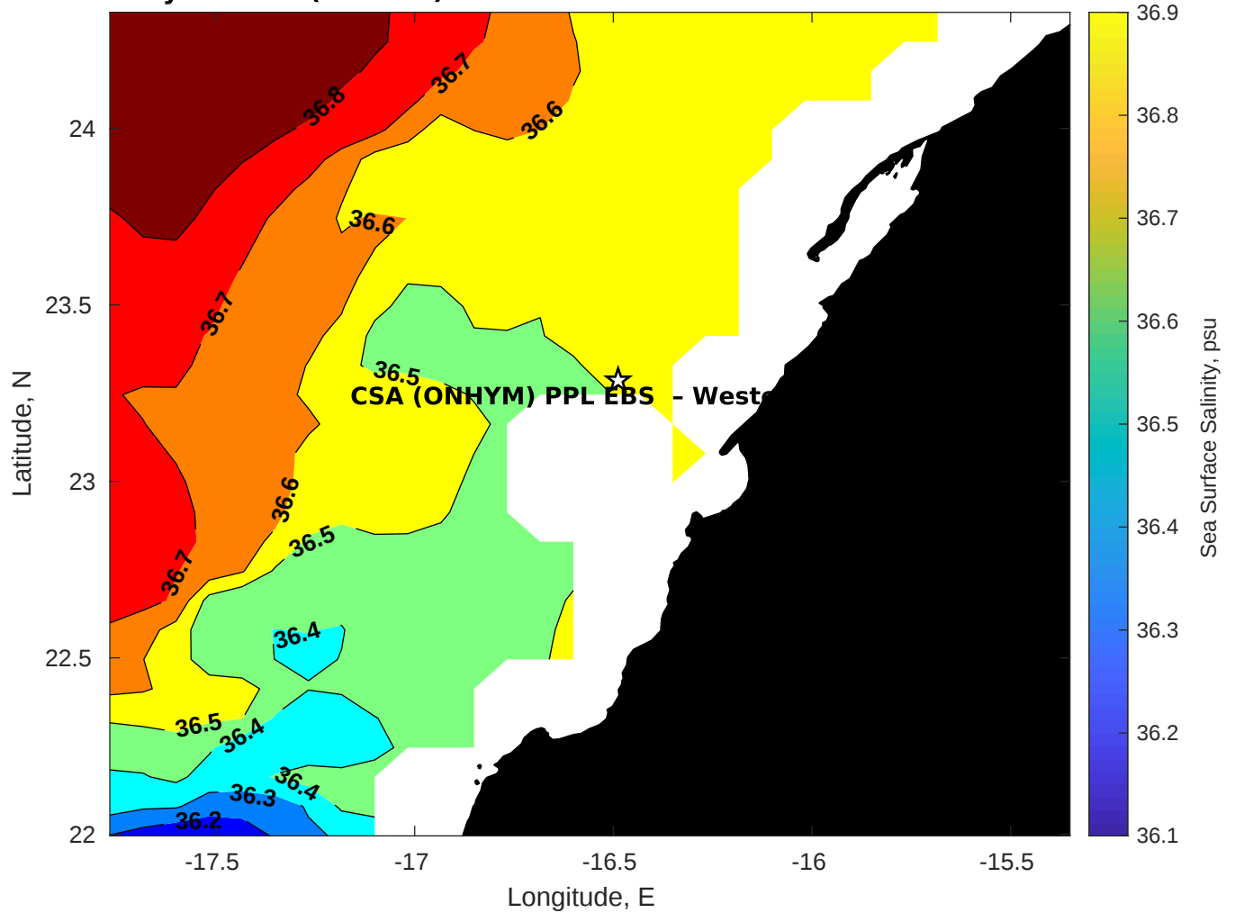
Surface Salinity for CSA (ONHYM) PPL EBS - Western Sahara at 25-Nov-2025 00:00:00
