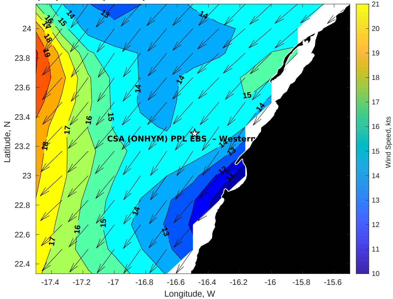
GFS Winds (kts) for CSA (ONHYM) PPL EBS - Western Sahara at 26-Nov-2025 09:00:00
