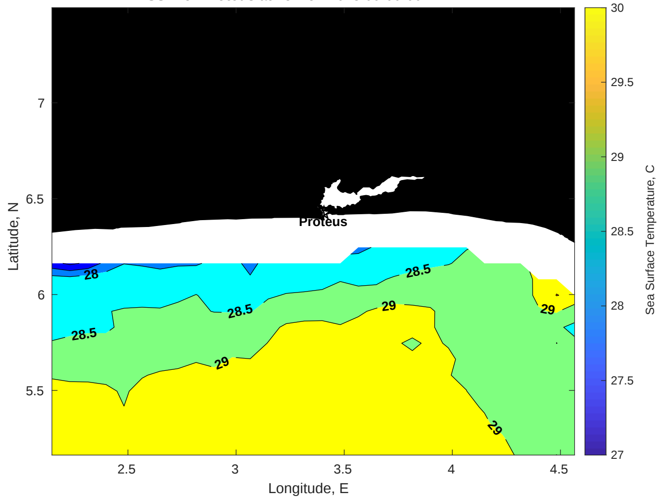
SST for Proteus at 25-Nov-2025 00:00:00
