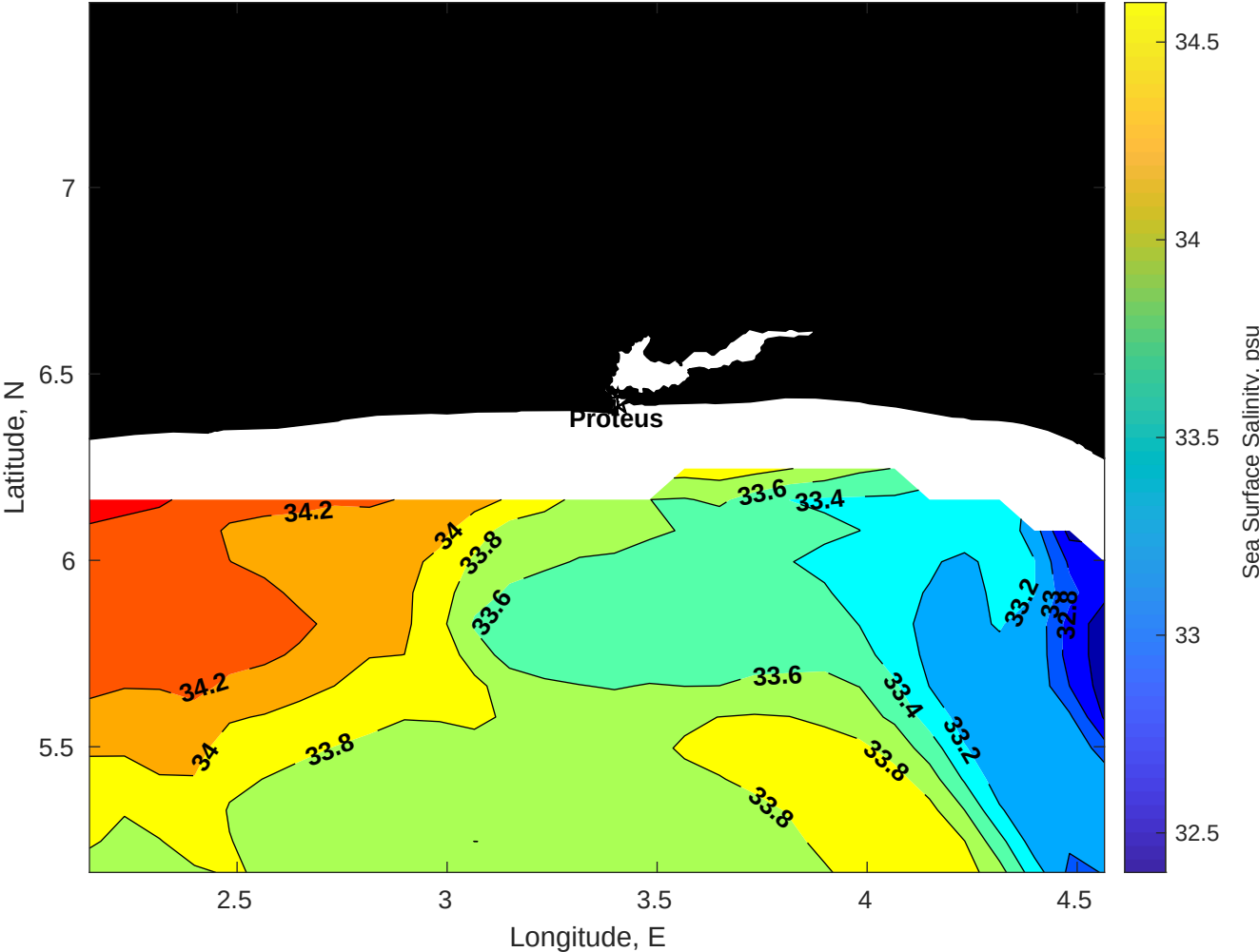
Surface Salinity for Proteus at 25-Nov-2025 00:00:00
