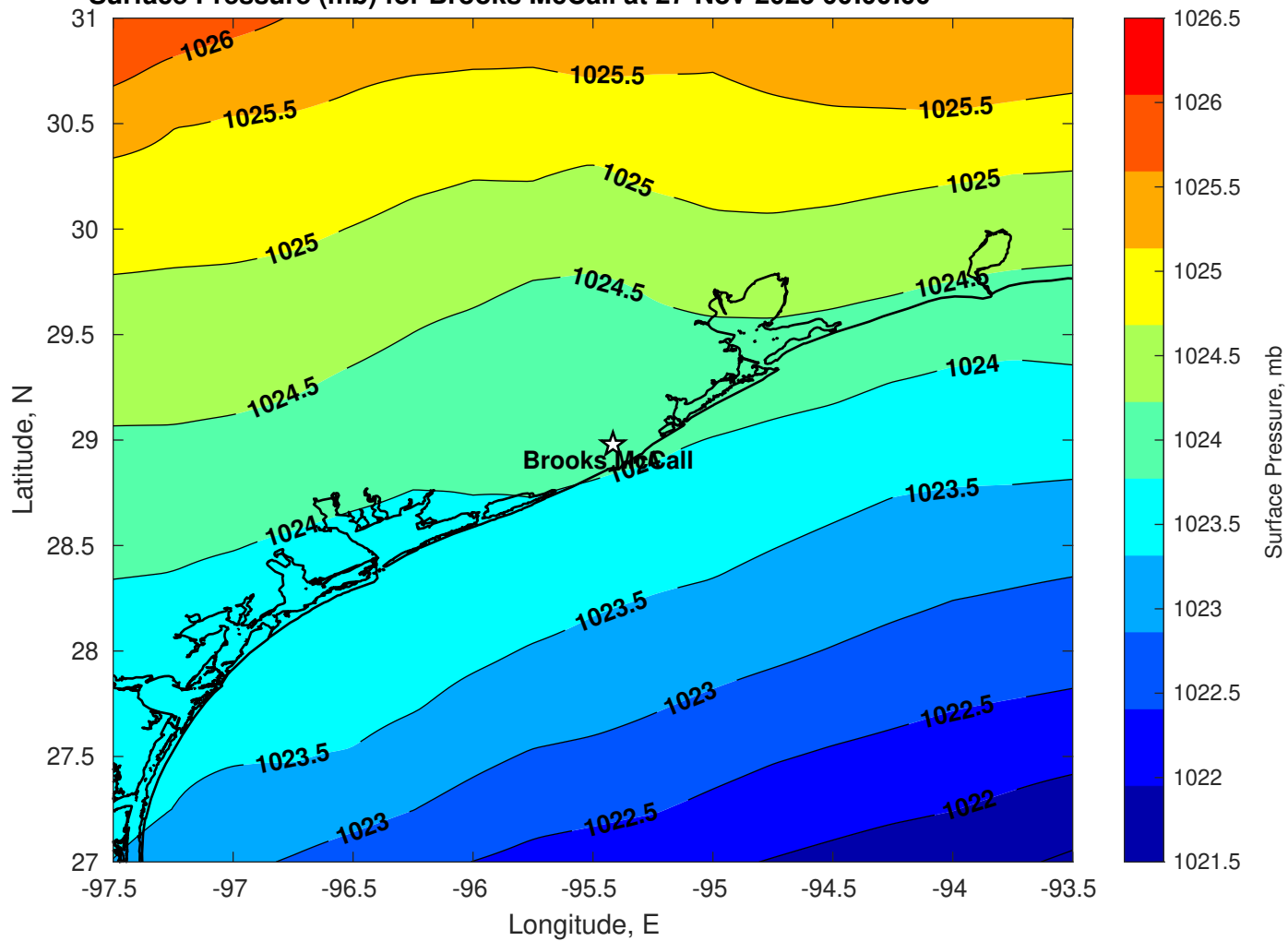
Surface Pressure (mb) for Brooks McCall at 27-Nov-2025 00:00:00
