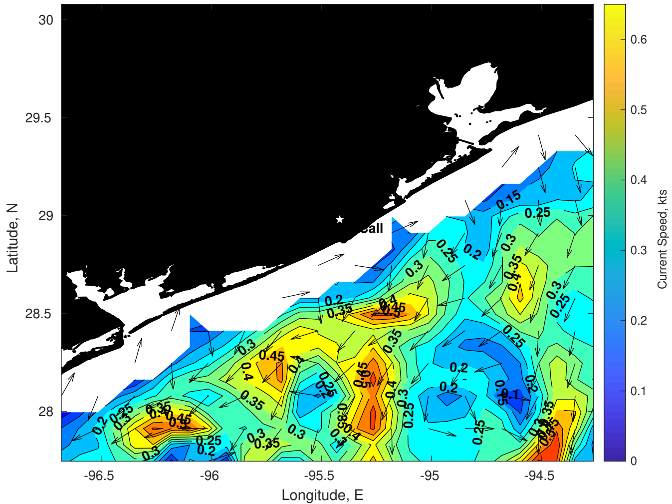
Surface Currents for Brooks McCall at 26-Nov-2025 00:00:00
