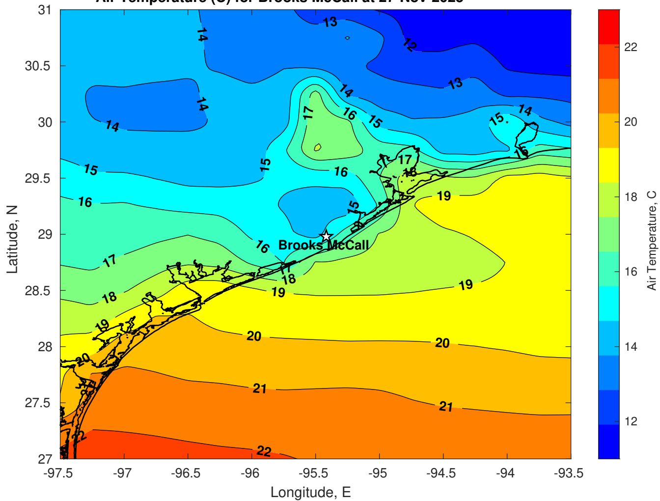
Air Temperature (C) for Brooks McCall at 27-Nov-2025
