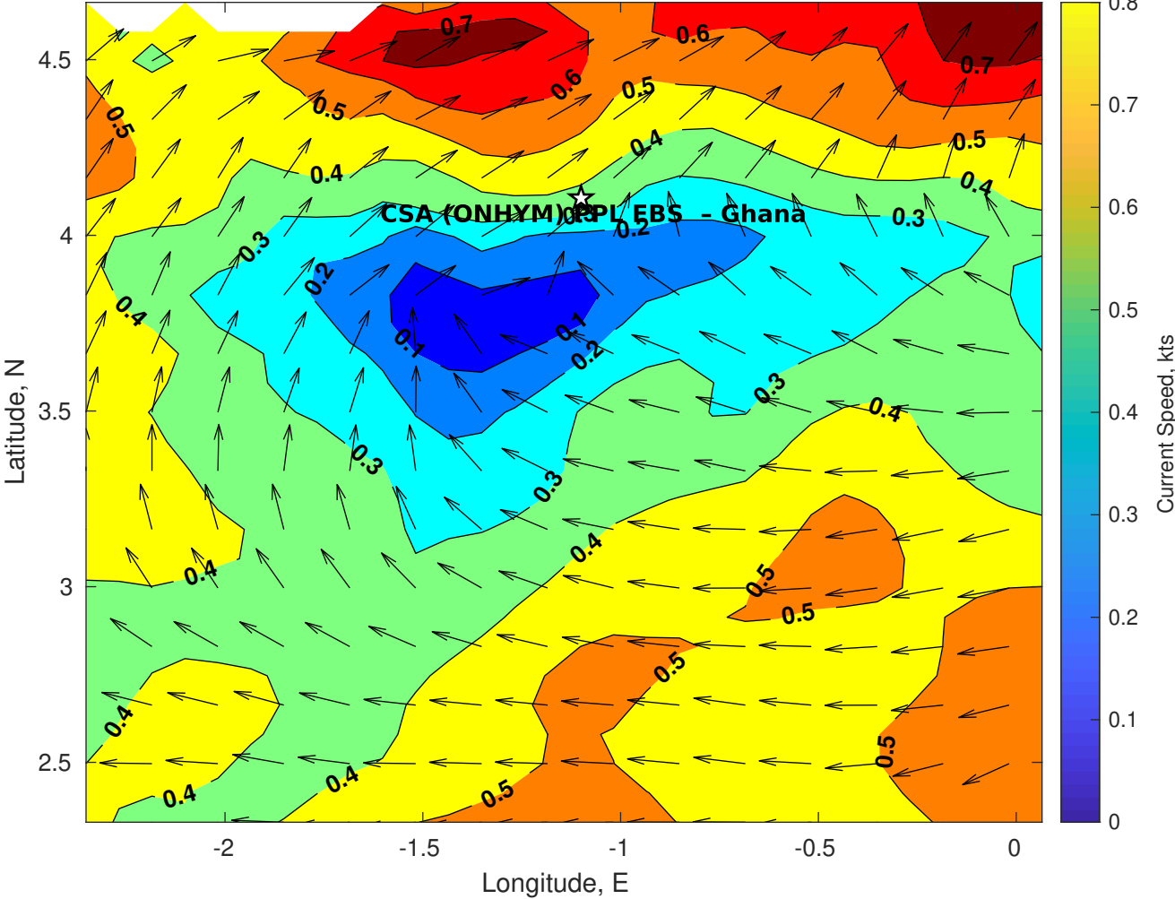
Surface Currents for CSA (ONHYM) PPL EBS - Ghana at 26-Nov-2025 00:00:00
