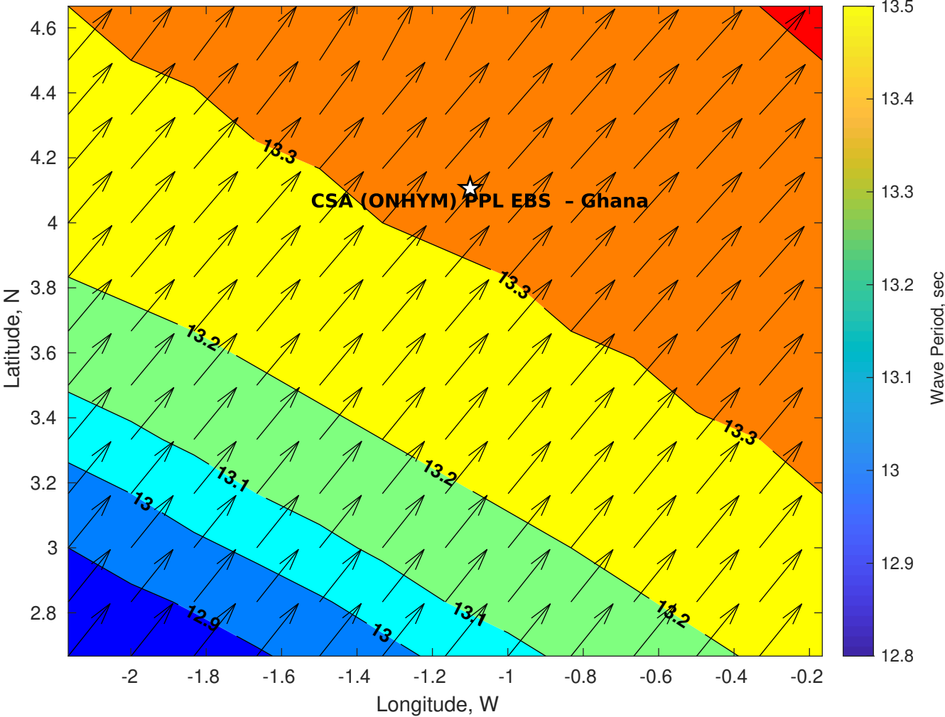
GFS Wave Period (sec) for CSA (ONHYM) PPL EBS - Ghana at 27-Nov-2025 09:00:00
