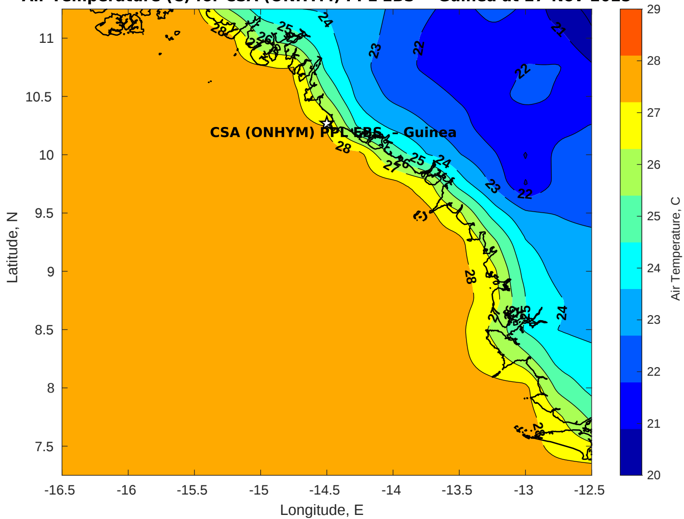
Air Temperature (C) for CSA (ONHYM) PPL EBS - Guinea at 27-Nov-2025
