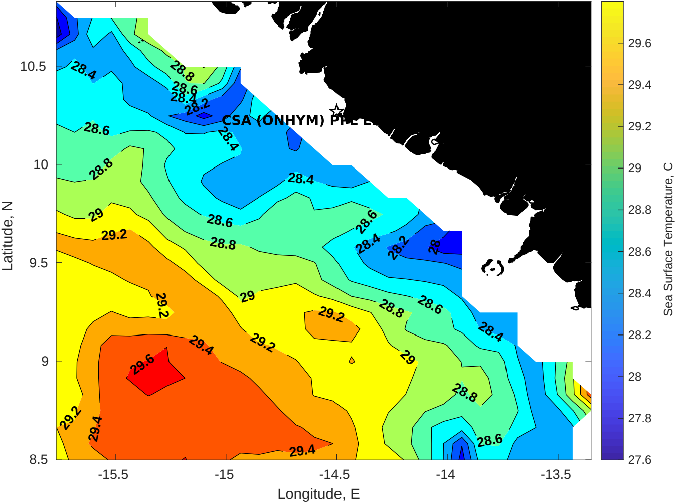
SST for CSA (ONHYM) PPL EBS - Guinea at 26-Nov-2025 00:00:00
