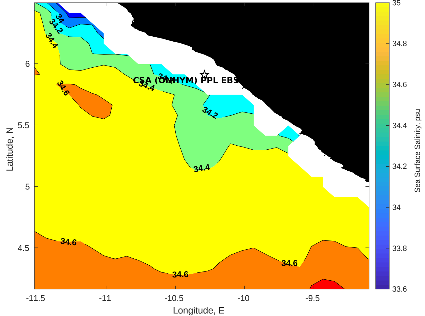
Surface Salinity for CSA (ONHYM) PPL EBS - Liberia at 26-Nov-2025 00:00:00
