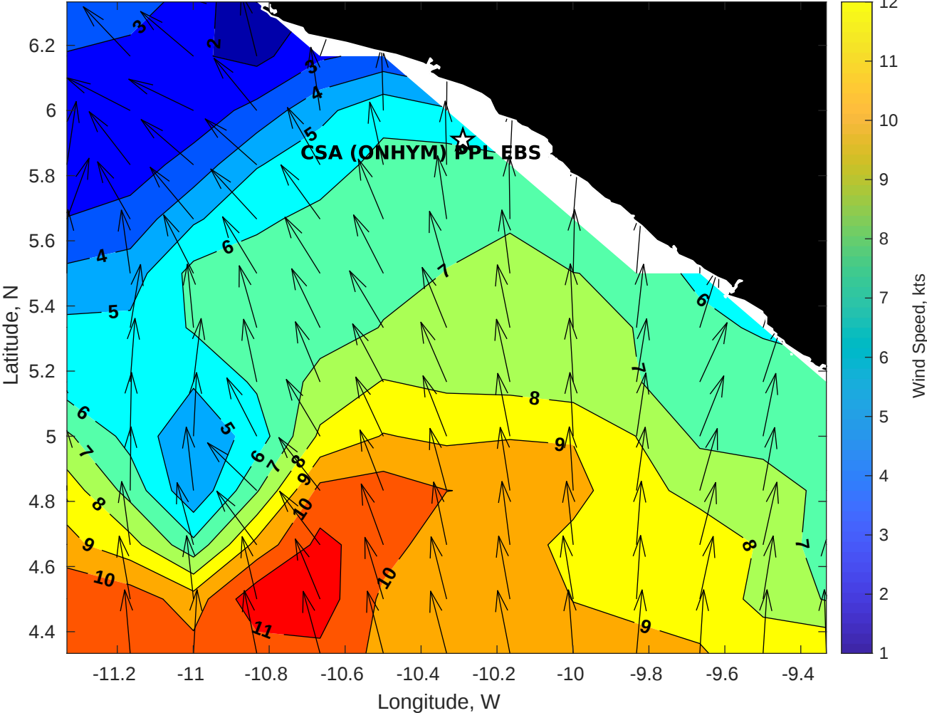
GFS Winds (kts) for CSA (ONHYM) PPL EBS - Liberia at 27-Nov-2025 09:00:00
