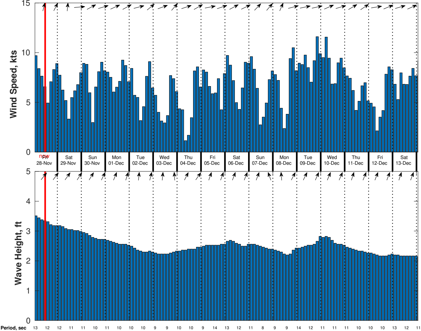
Wind & Wave Forecast for CSA (ONHYM) PPL EBS - Liberia from 27-Nov-2025 01:00:00 to 13-Dec-2025 01:00:00
