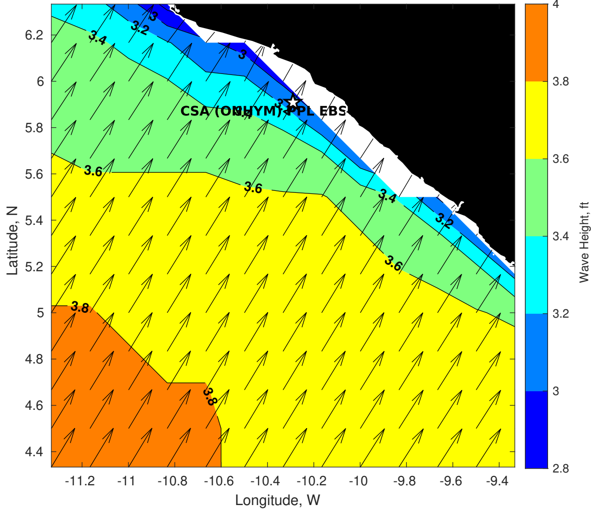
GFS Wave Height (ft) for CSA (ONHYM) PPL EBS - Liberia at 27-Nov-2025 09:00:00
