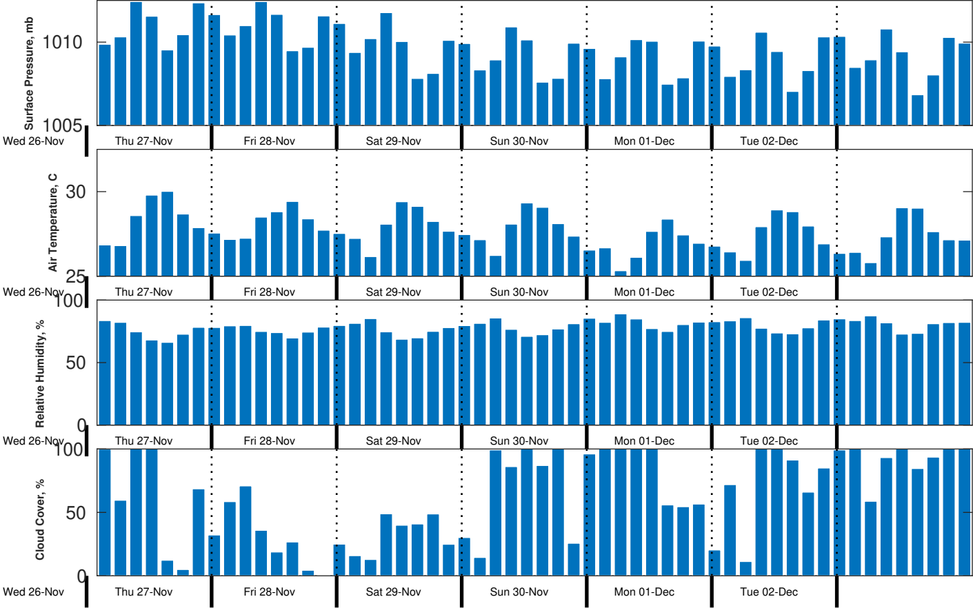
Met Forecast for CSA (ONHYM) PPL EBS - Liberia from 27-Nov-2025 00:00:00 to 04-Dec-2025 00:00:00
