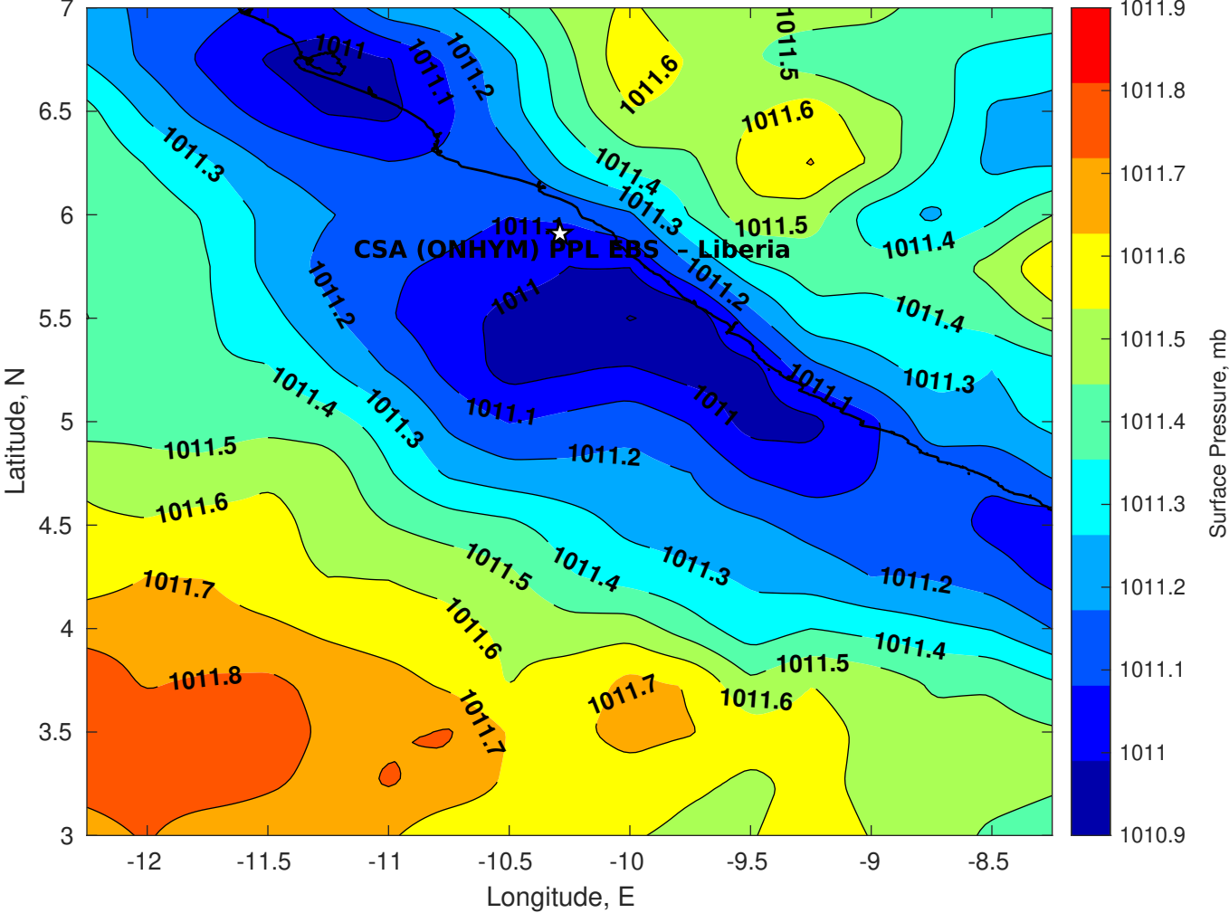
Surface Pressure (mb) for CSA (ONHYM) PPL EBS - Liberia at 29-Nov-2025 00:00:00
