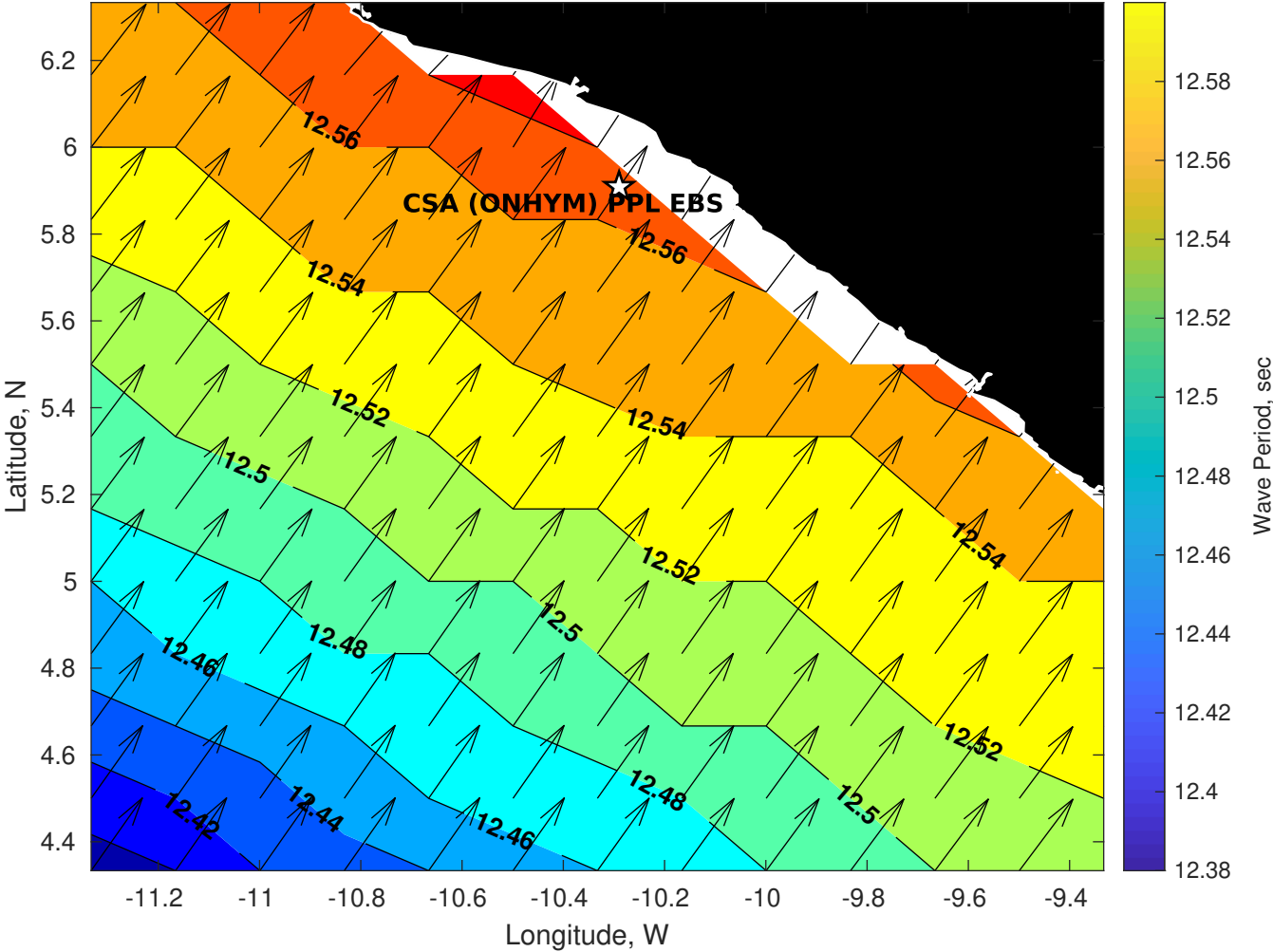
GFS Wave Period (sec) for CSA (ONHYM) PPL EBS - Liberia at 27-Nov-2025 09:00:00
