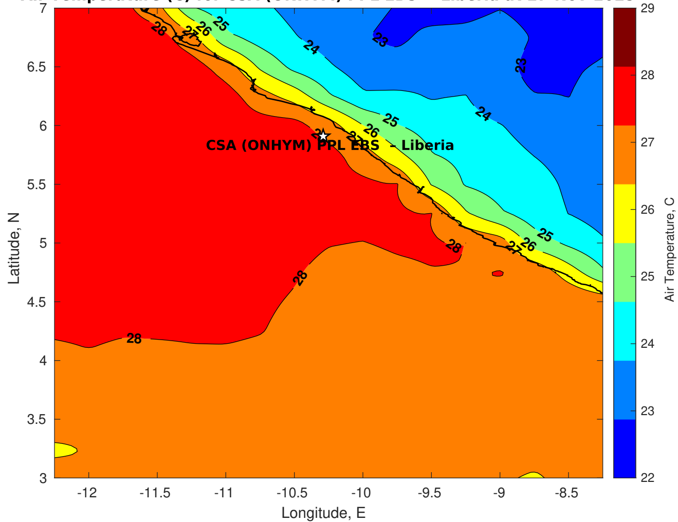
Air Temperature (C) for CSA (ONHYM) PPL EBS - Liberia at 27-Nov-2025
