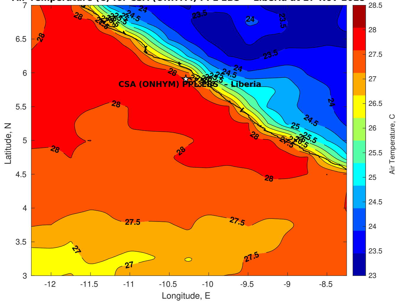
Air Temperature (C) for CSA (ONHYM) PPL EBS - Liberia at 27-Nov-2025
