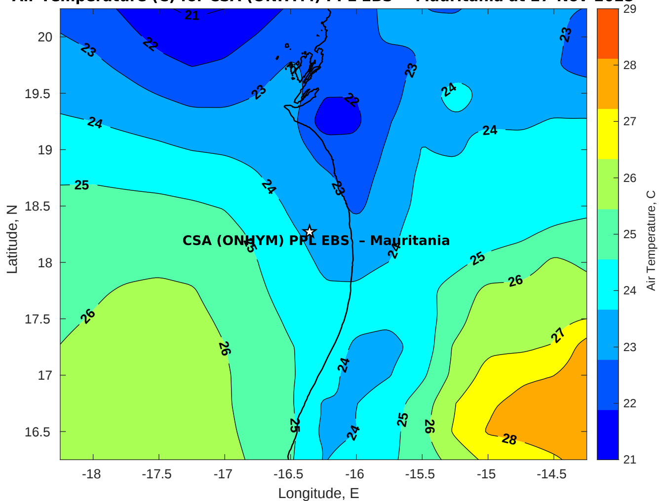
Air Temperature (C) for CSA (ONHYM) PPL EBS - Mauritania at 27-Nov-2025
