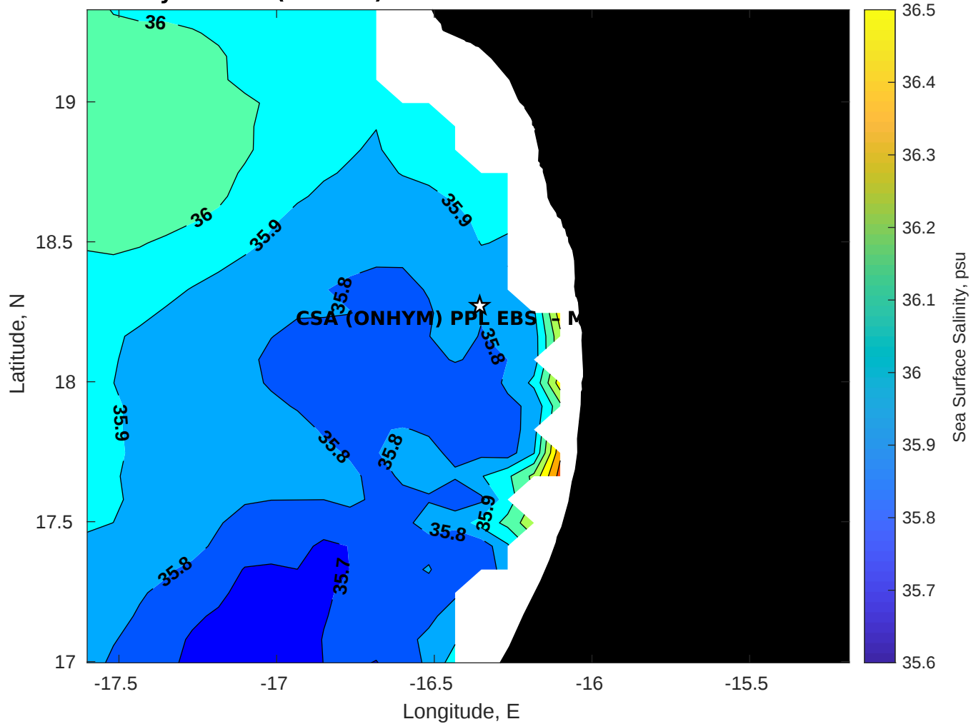
Surface Salinity for CSA (ONHYM) PPL EBS - Mauritania at 26-Nov-2025 00:00:00
