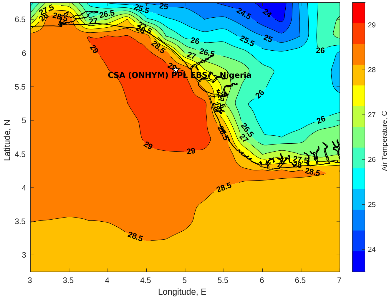
Air Temperature (C) for CSA (ONHYM) PPL EBS - Nigeria at 27-Nov-2025
