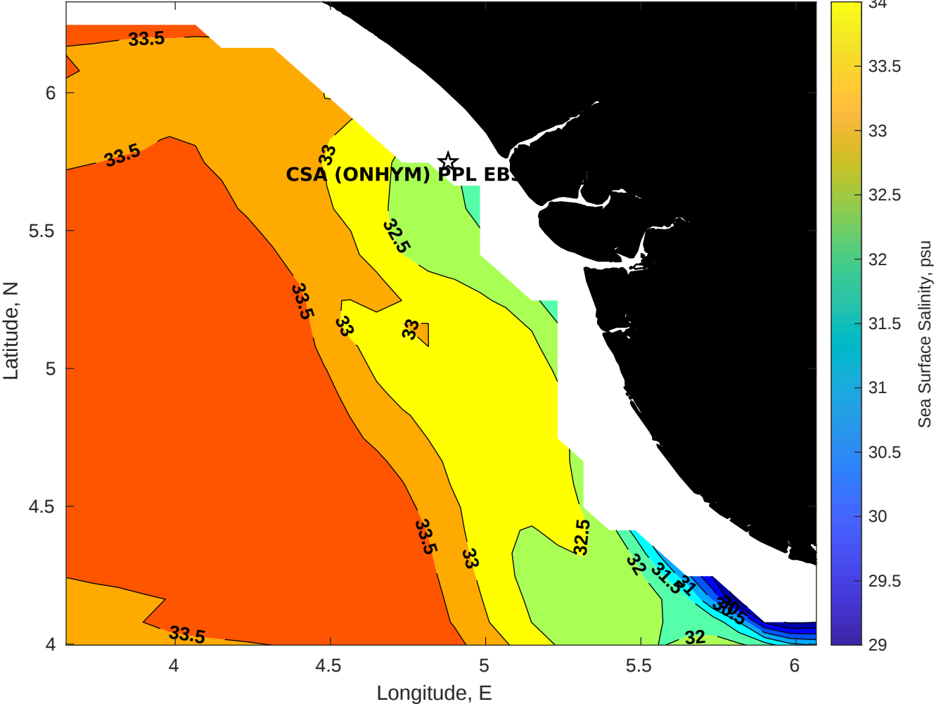
Surface Salinity for CSA (ONHYM) PPL EBS - Nigeria at 26-Nov-2025 00:00:00
