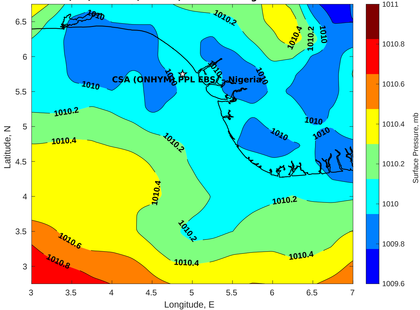
Surface Pressure (mb) for CSA (ONHYM) PPL EBS - Nigeria at 28-Nov-2025 00:00:00
