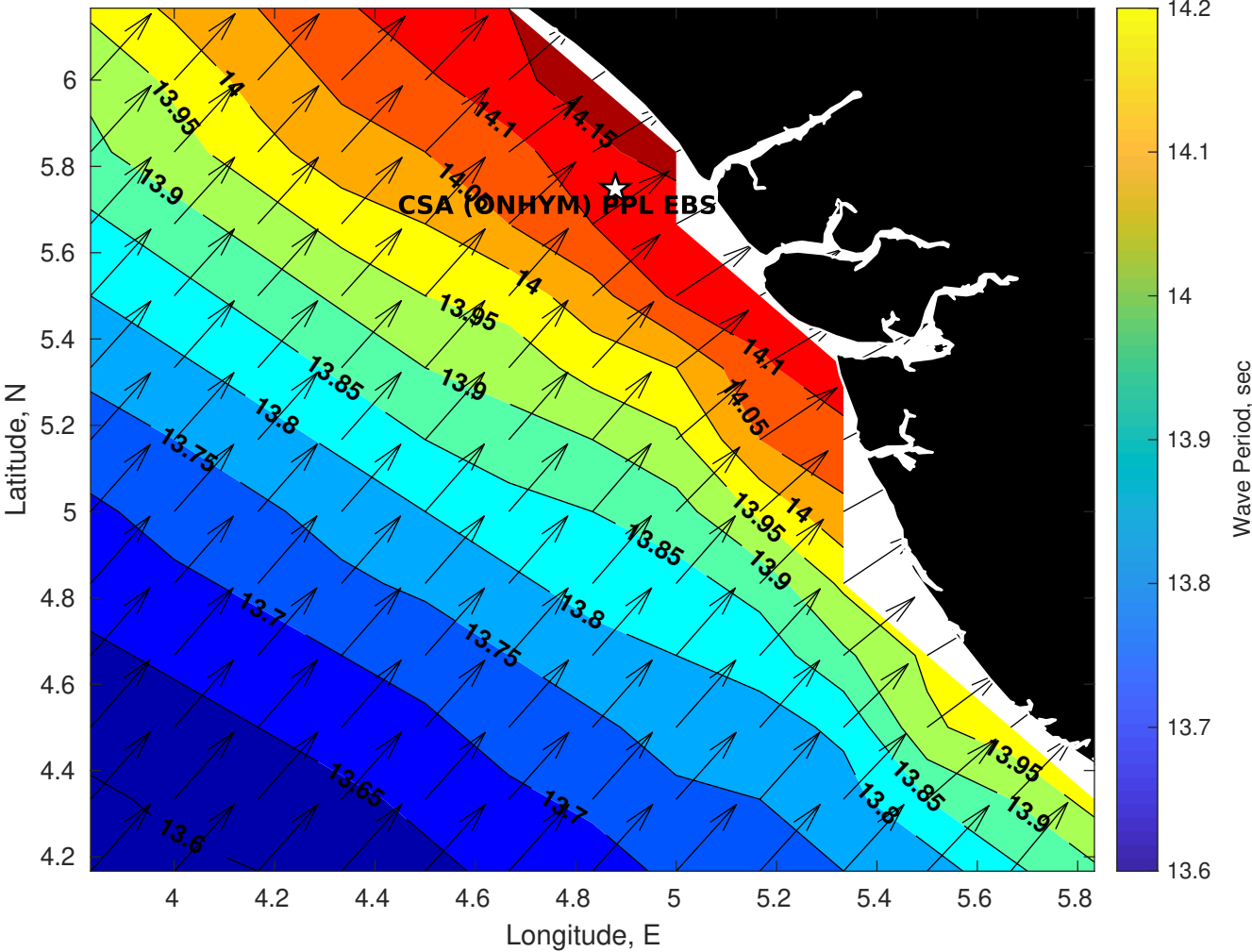
GFS Wave Period (sec) for CSA (ONHYM) PPL EBS - Nigeria at 27-Nov-2025 09:00:00
