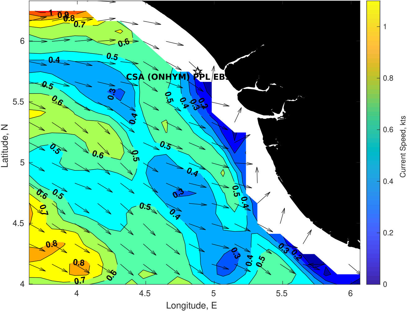
Surface Currents for CSA (ONHYM) PPL EBS - Nigeria at 26-Nov-2025 00:00:00
