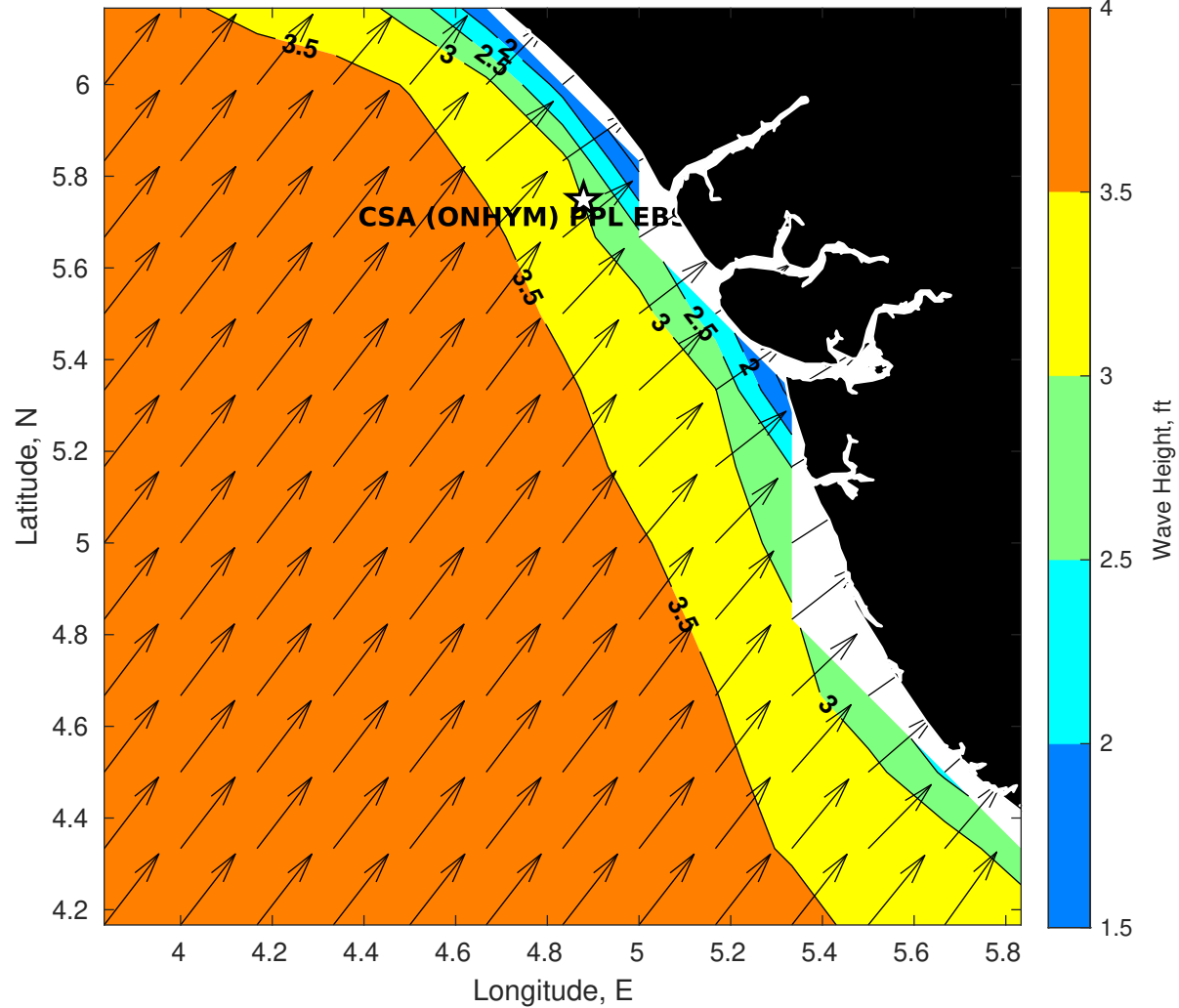
GFS Wave Height (ft) for CSA (ONHYM) PPL EBS - Nigeria at 27-Nov-2025 09:00:00
