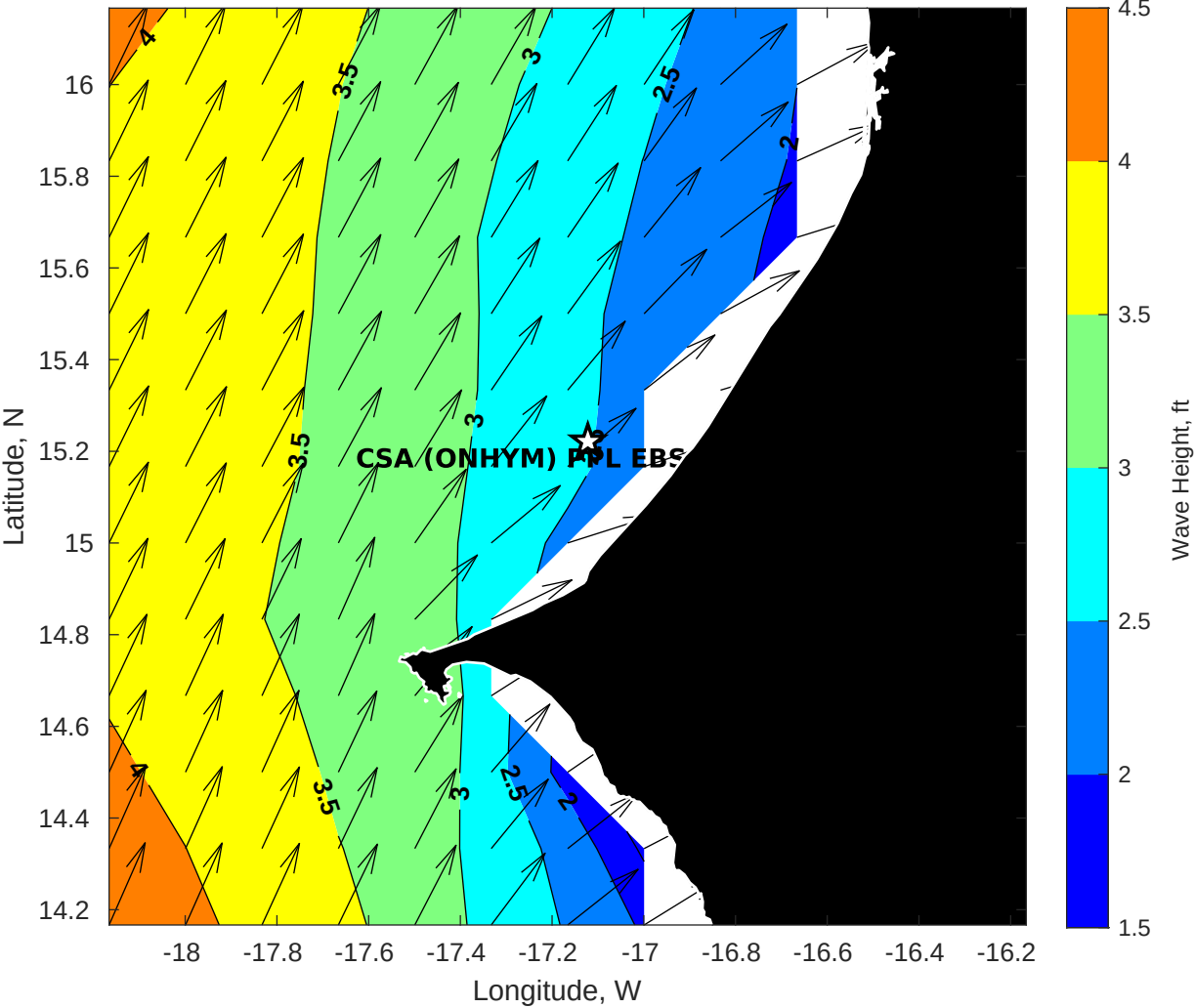
GFS Wave Height (ft) for CSA (ONHYM) PPL EBS - Senegal at 27-Nov-2025 09:00:00
