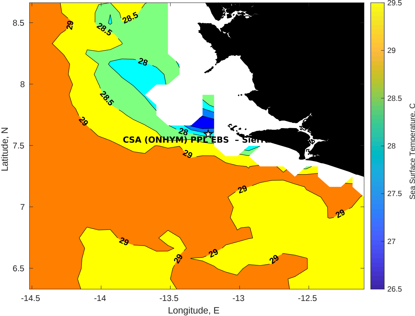
SST for CSA (ONHYM) PPL EBS - Sierra Leone at 26-Nov-2025 00:00:00
