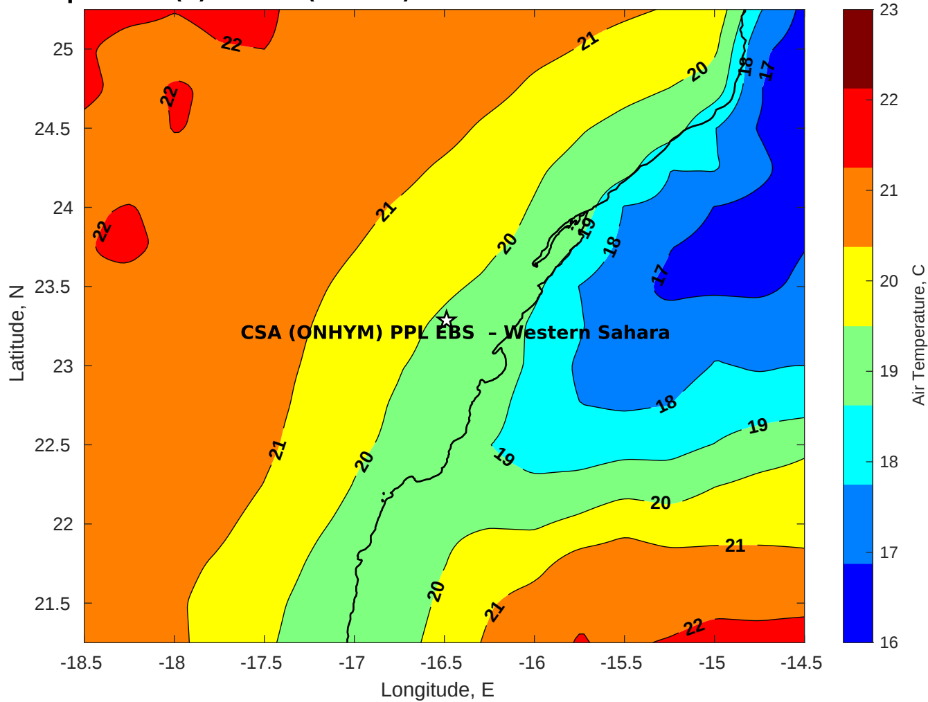
Air Temperature (C) for CSA (ONHYM) PPL EBS - Western Sahara at 27-Nov-2025
