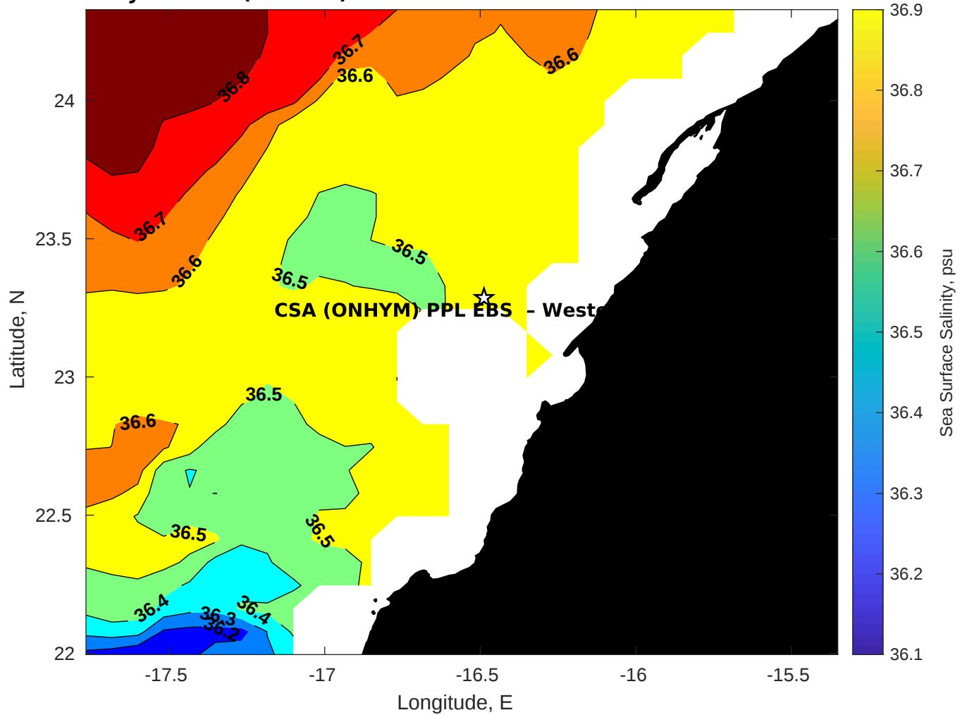
Surface Salinity for CSA (ONHYM) PPL EBS - Western Sahara at 26-Nov-2025 00:00:00
