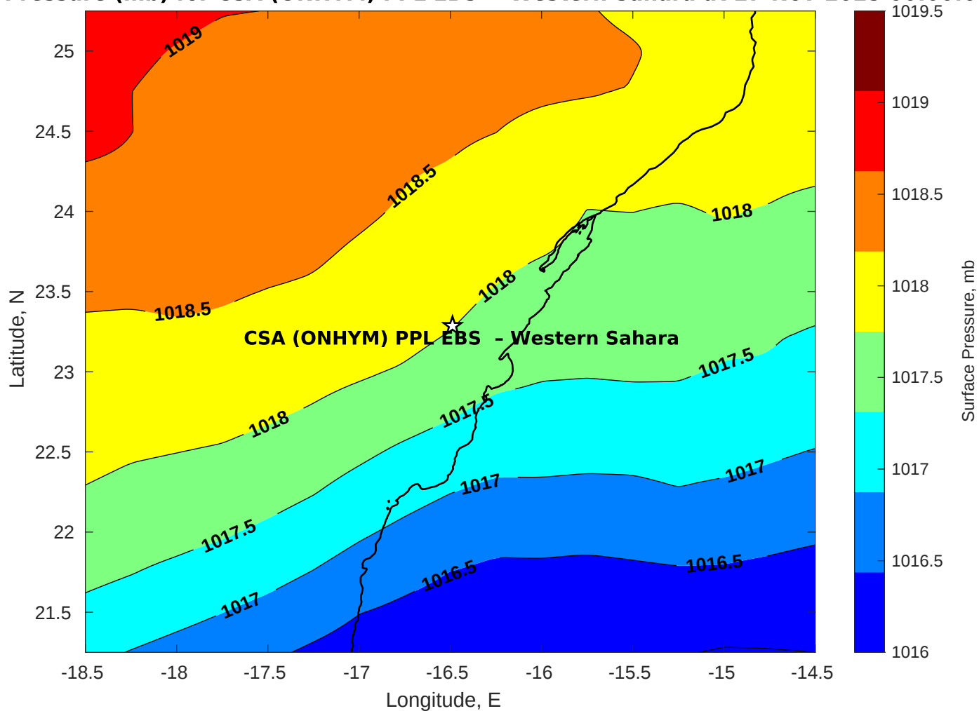
Surface Pressure (mb) for CSA (ONHYM) PPL EBS - Western Sahara at 27-Nov-2025 00:00:00
