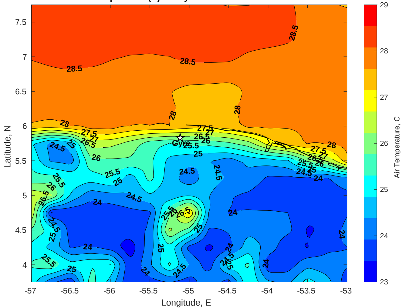
Air Temperature (C) for Gyre at 27-Nov-2025
