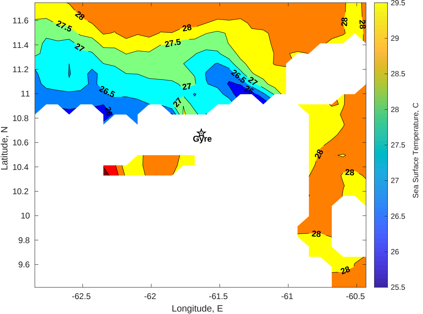
SST for Gyre at 26-Nov-2025 00:00:00
