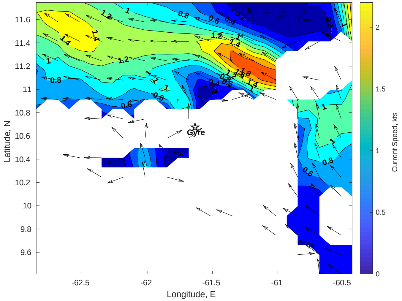
Surface Currents for Gyre at 26-Nov-2025 00:00:00
