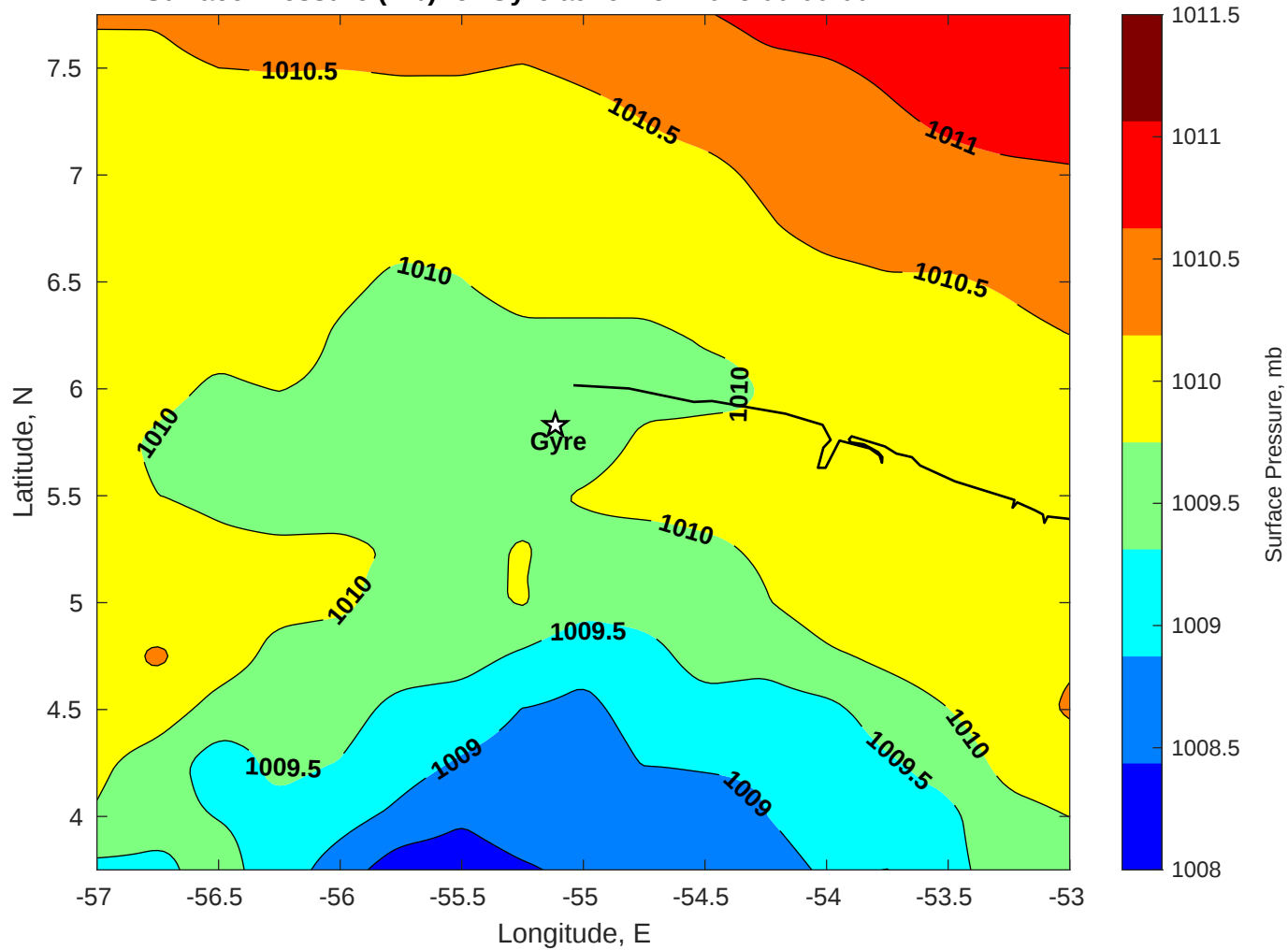
Surface Pressure (mb) for Gyre at 29-Nov-2025 00:00:00
