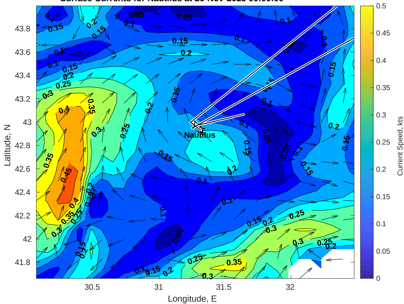
Surface Currents for Nautilus at 26-Nov-2025 00:00:00
