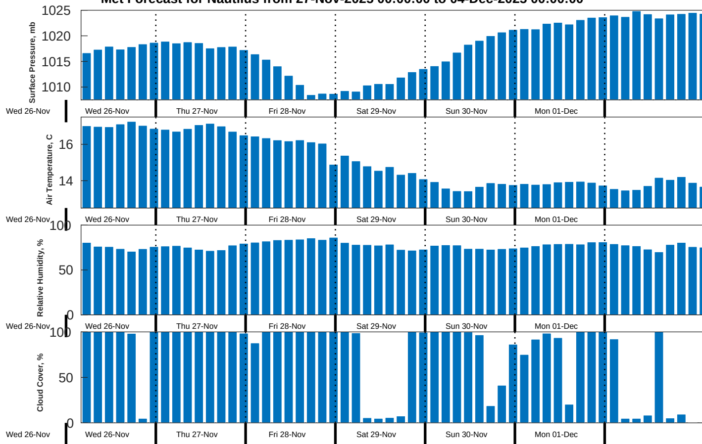
Met Forecast for Nautilus from 27-Nov-2025 00:00:00 to 04-Dec-2025 00:00:00
