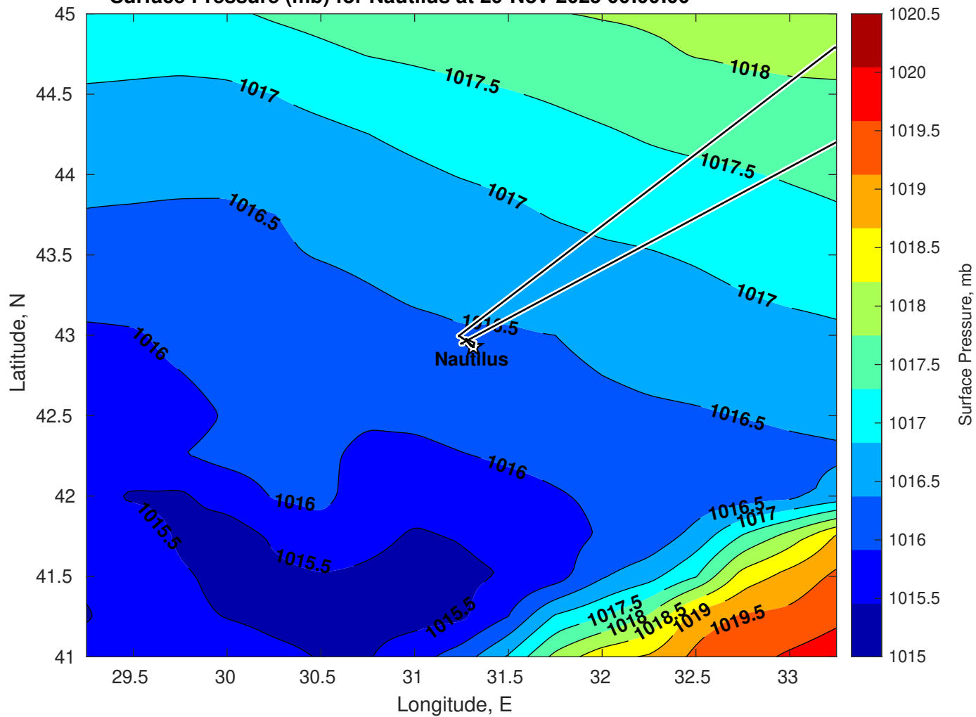
Surface Pressure (mb) for Nautilus at 29-Nov-2025 00:00:00
