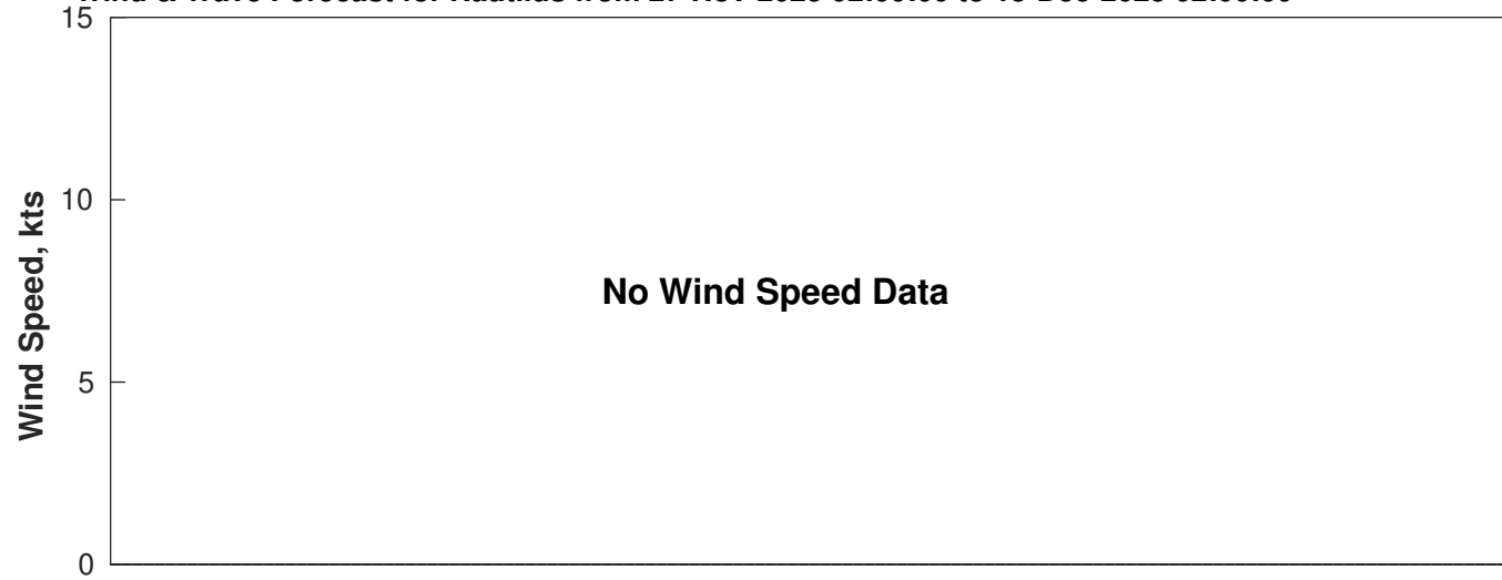
Wind & Wave Forecast for Nautilus from 27-Nov-2025 02:00:00 to 13-Dec-2025 02:00:00
