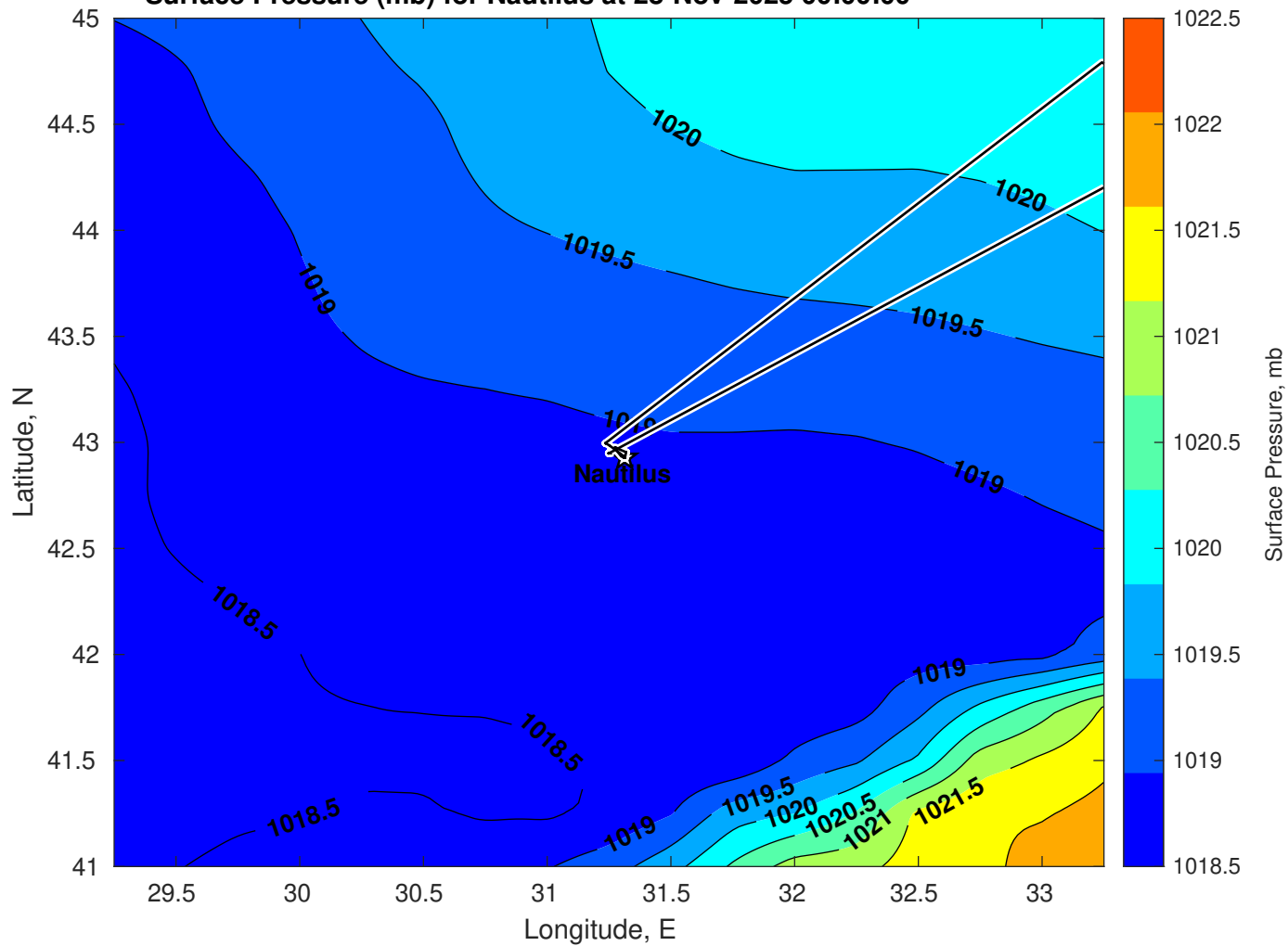
Surface Pressure (mb) for Nautilus at 28-Nov-2025 00:00:00
