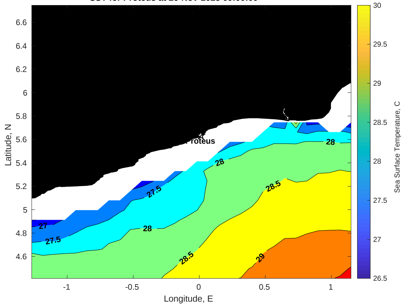
SST for Proteus at 26-Nov-2025 00:00:00
