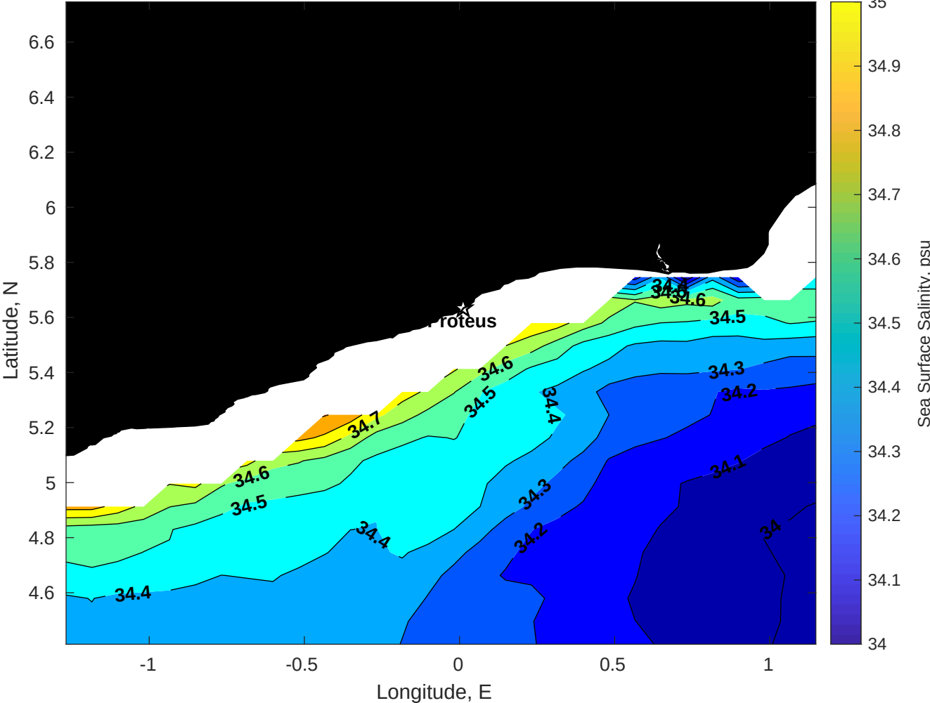
Surface Salinity for Proteus at 26-Nov-2025 00:00:00
