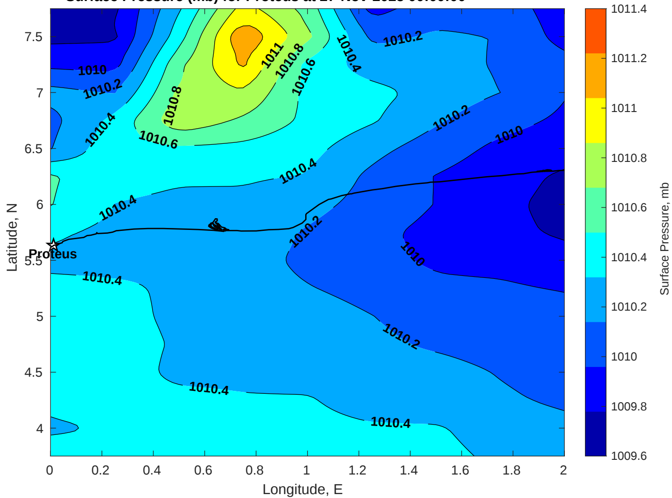
Surface Pressure (mb) for Proteus at 27-Nov-2025 00:00:00
