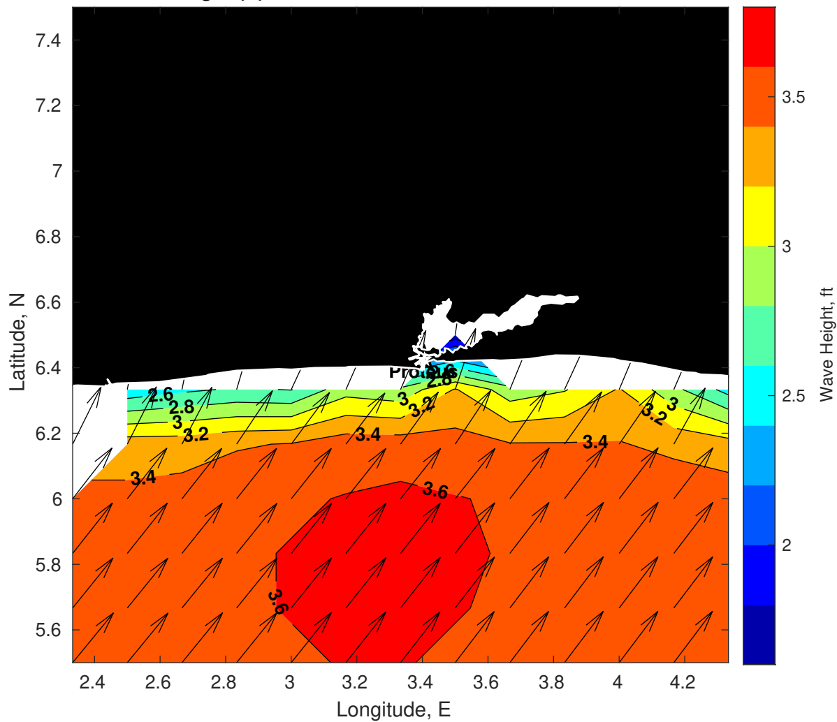
GFS Wave Height (ft) for Proteus at 25-Nov-2025 21:00:00
