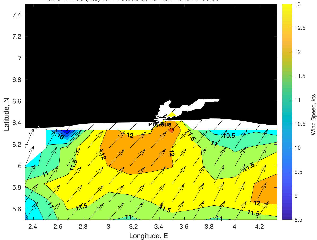
GFS Winds (kts) for Proteus at 25-Nov-2025 21:00:00
