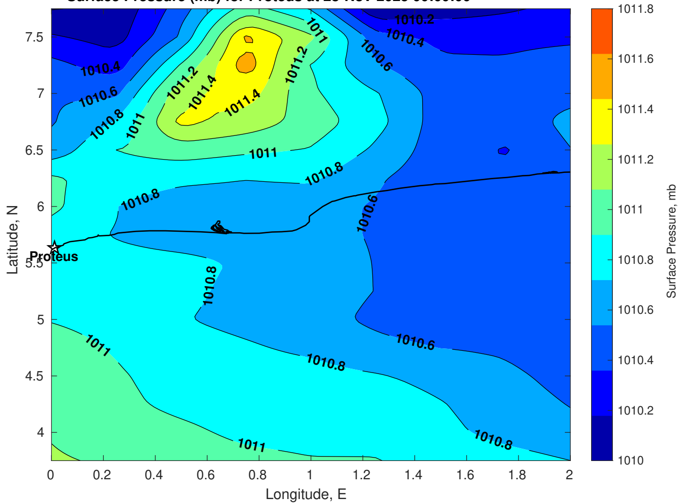
Surface Pressure (mb) for Proteus at 28-Nov-2025 00:00:00
