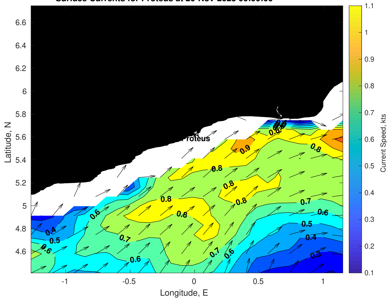
Surface Currents for Proteus at 26-Nov-2025 00:00:00
