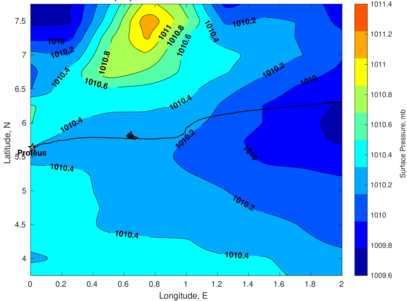
Surface Pressure (mb) for Proteus at 27-Nov-2025 00:00:00
