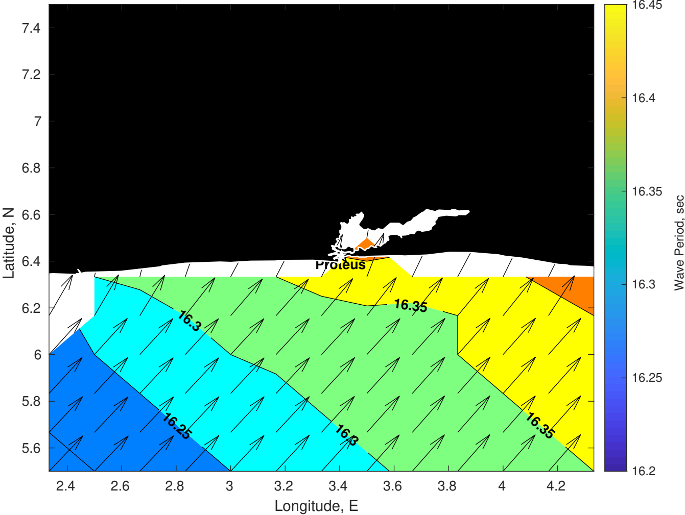
GFS Wave Period (sec) for Proteus at 25-Nov-2025 21:00:00
