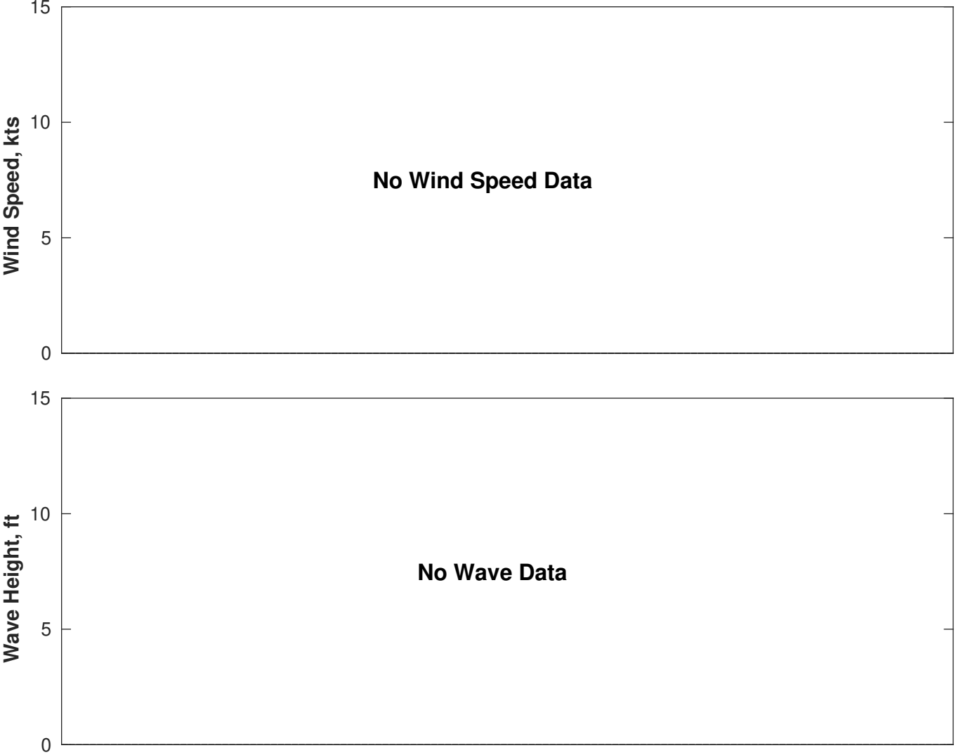
Wind & Wave Forecast for Proteus from 27-Nov-2025 01:00:00 to 13-Dec-2025 01:00:00
