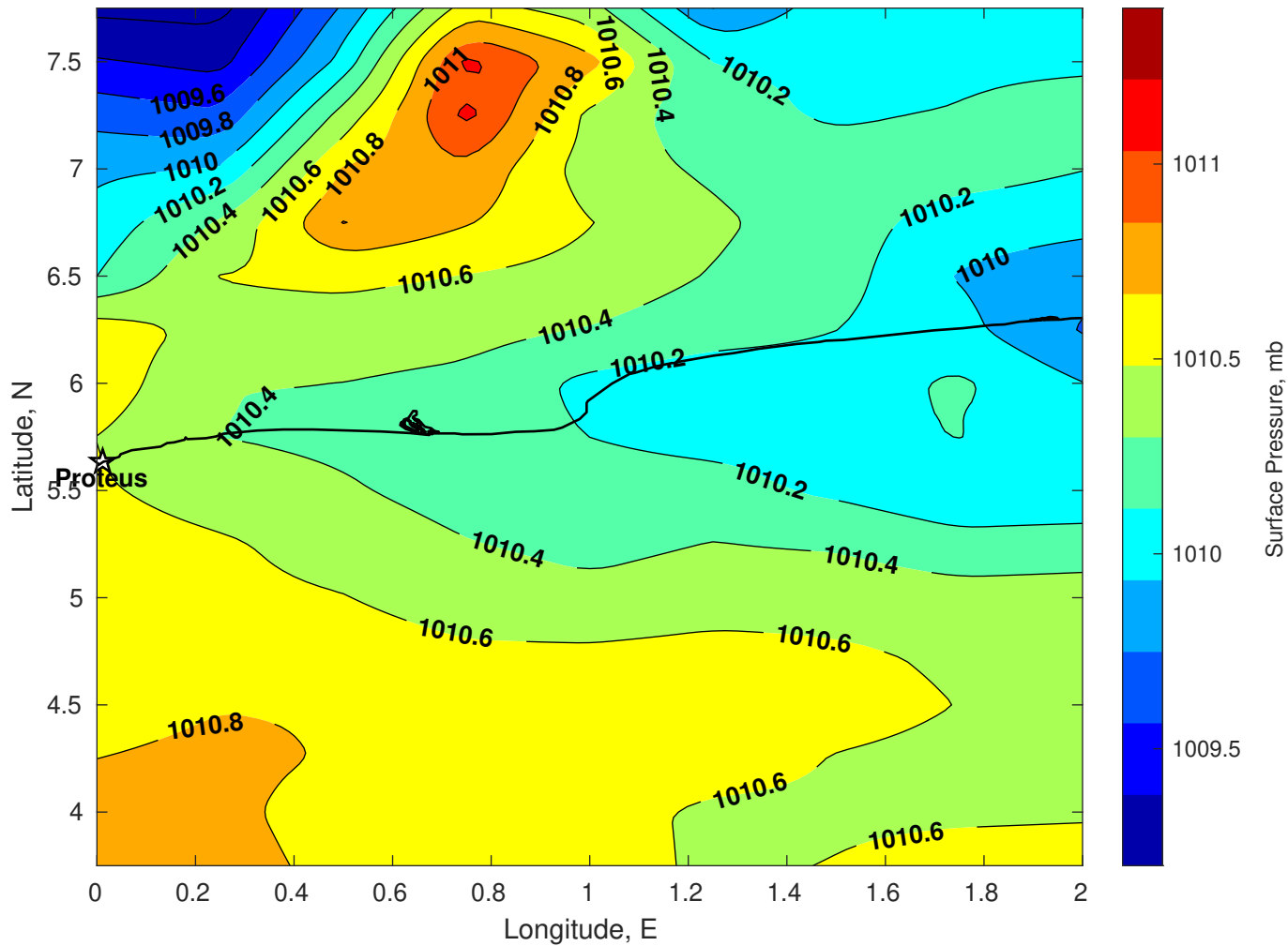
Surface Pressure (mb) for Proteus at 29-Nov-2025 00:00:00
