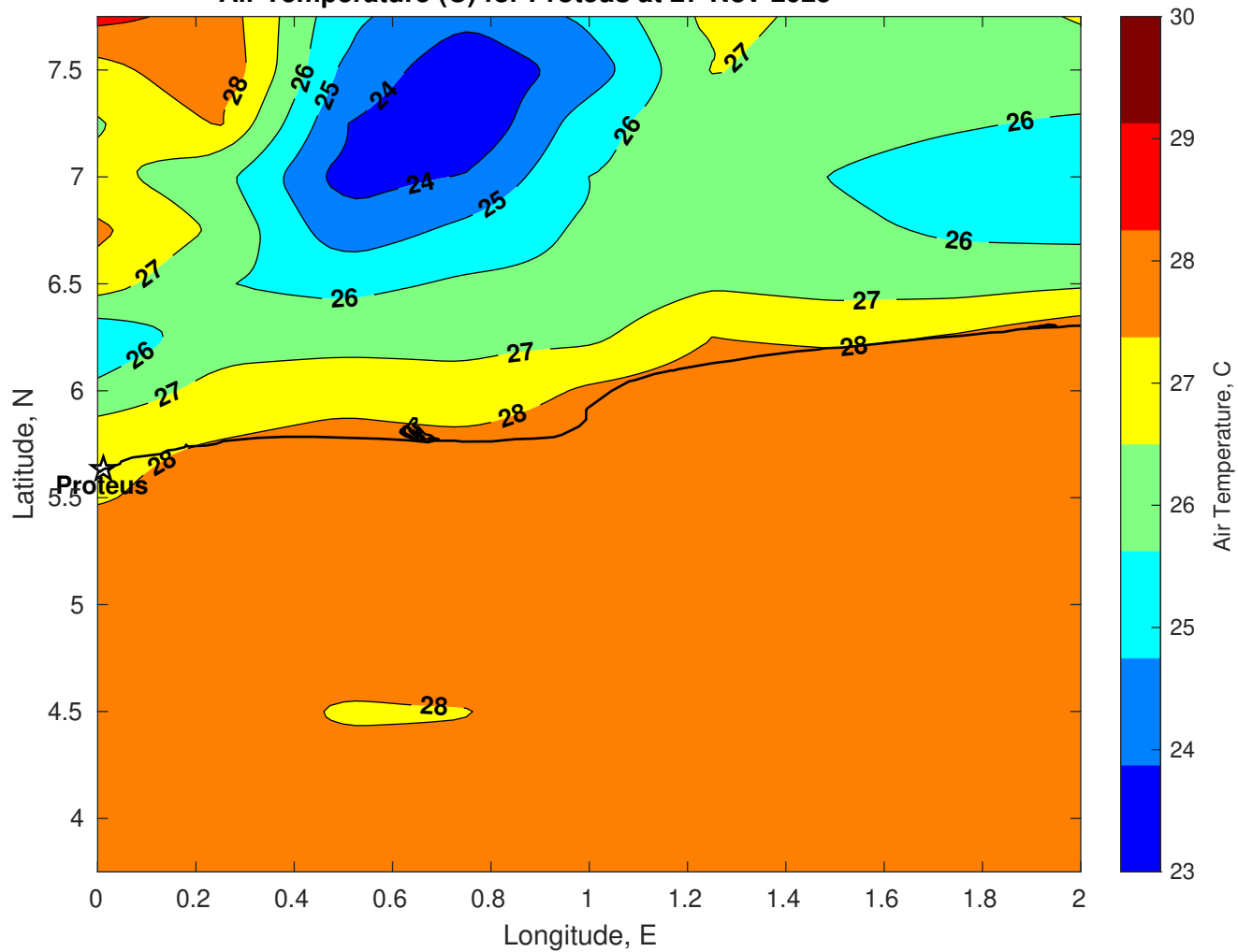
Air Temperature (C) for Proteus at 27-Nov-2025
