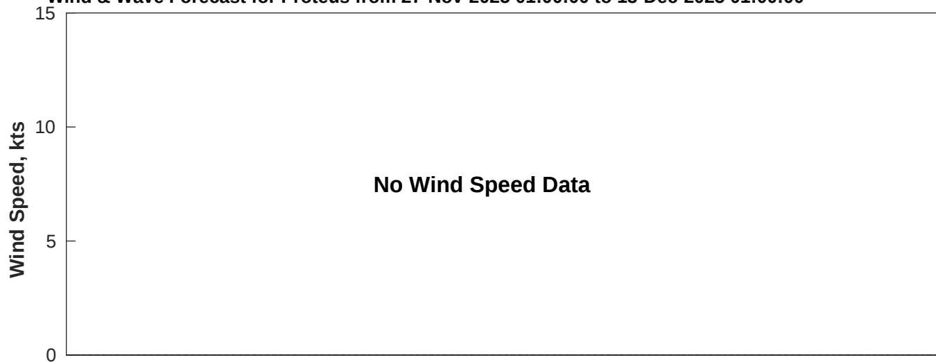
Wind & Wave Forecast for Proteus from 27-Nov-2025 01:00:00 to 13-Dec-2025 01:00:00
