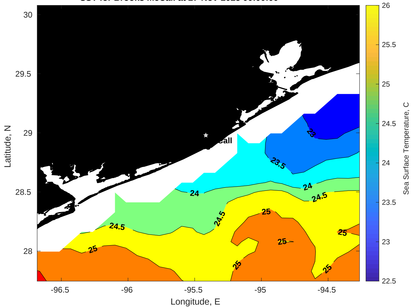
SST for Brooks McCall at 27-Nov-2025 00:00:00
